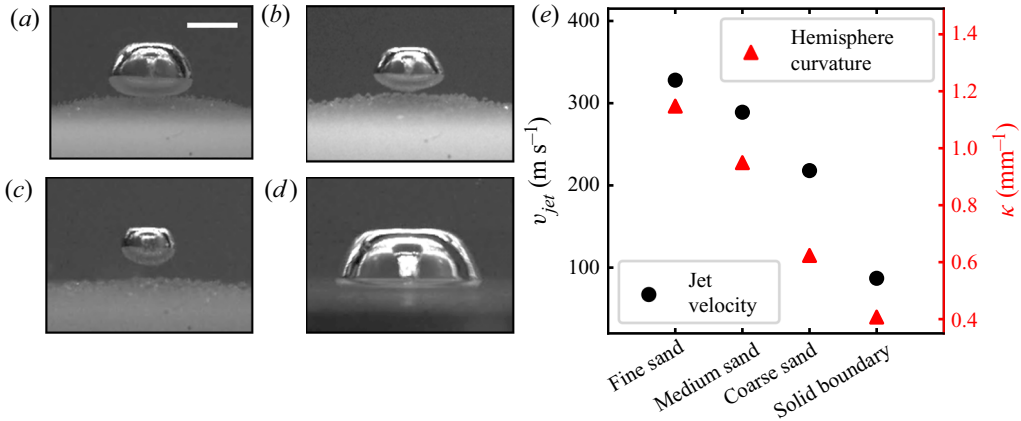
Figure 8. Observation of the micro-jets driven by the nearby boundaries at \gamma \approx 0.8 : (a) fine sand ( d_g = 90 \mu m ), (b) medium sand ( d_g = 200 \mu m ), (c) coarse sand ( d_g = 350 \mu m ) and (d) rigid boundary. The white line indicates the 2 mm scale. (e) The associated averaged jet speeds measured between jet formation and opposite bubble wall impact, and the curvatures of the bubbles upper hemispheres measured before the micro-jet formation.
