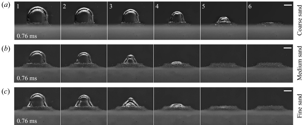
Figure 10. Final phase of the bubble collapse near the different granular boundaries at \gamma \approx 0.5 : (a) coarse sand ( d_g = 350 \mu\text{m} ), (b) medium sand ( d_g = 200 \mu\text{m} ) and (c) fine sand ( d_g = 90 \mu\text{m} ). All image sequences are initiated 0.76 ms after the bubble generation and the time interval between successive images is 20 \mu\text{s} . The white line indicates the 2 mm scale.
