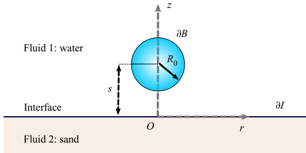
Figure 3. Schematic of the numerical domain.
