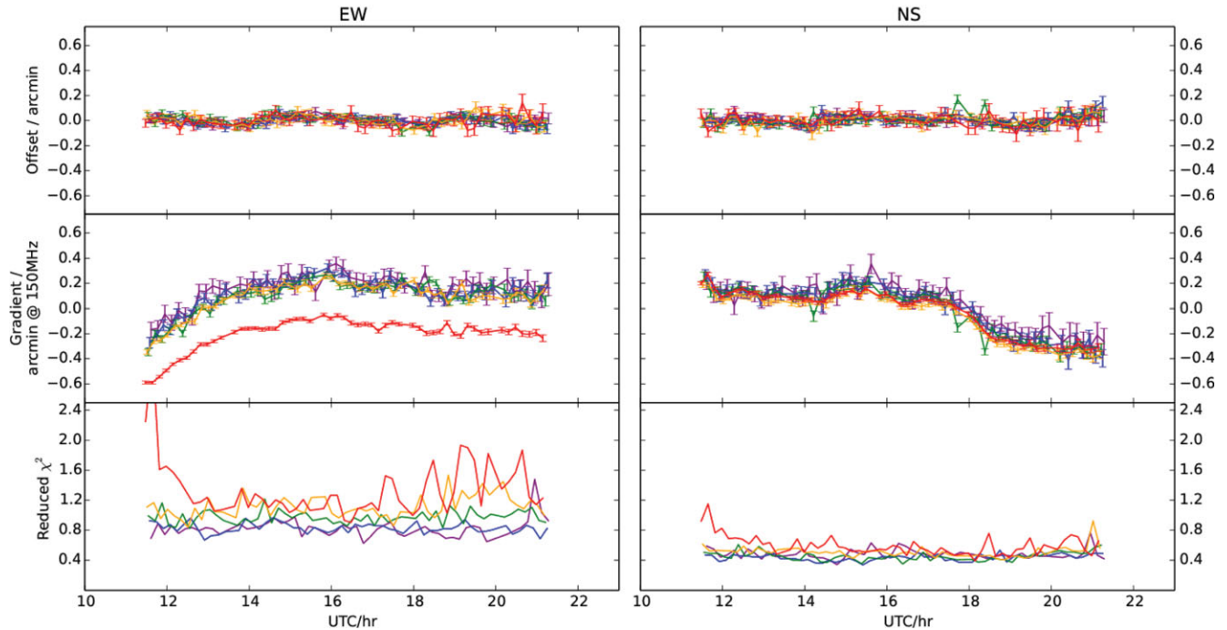
Figure 7. Offset (extrapolated to \lambda = 0 ), gradient, and reduced \chi^2 of a fit of source position offset as a function of \lambda^2 . Each point is for a single observation, all quantities are averaged over all (100) sources detected in that observation. Left panels are for the EW position offset (Right Ascension) right panels are for the NS position offset (Declination). Red, yellow, green, blue, and purple are for the 88, 118, 154, 185, and 215 MHz bands, respectively. Note that the gradients (in \text{arcmin m}^{-1} ) have been multiplied by 4, representing an offset at a wavelength of 2 m (=150 MHz).
