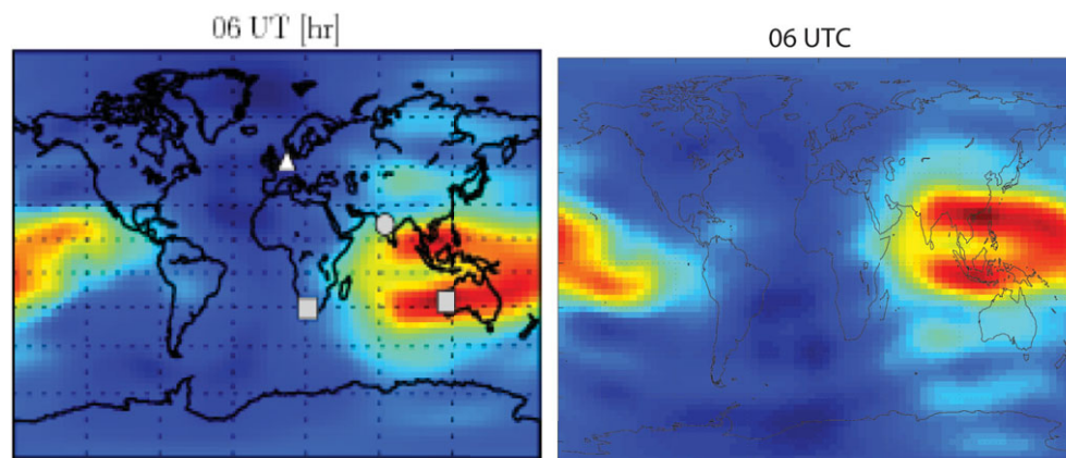
(a) CODE IONEX plot in Sotomayor-Beltran et al. (2013) (b) CODE IONEX plot by our software
