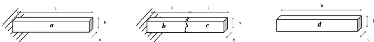
Fig. 6. Representation of boundary conditions in different configurations. (a) For a clamped beam and vibrations propagating in the along-flow direction, \frac{U(x_0)}{dx} = 0, x = x_0 . (b) Then we consider the ice tongue as two beams separated by the rift in the middle. We obtain two beams, one clamped and the other on the front of the glacier and simply supported. For a clamped beam on the first part, \frac{U(x_0)}{dx} = 0, x = x_0 . (c) For a simply supported free-end beam on the second part, \frac{d^2U}{dx^2} = 0, x = x_0 . (d) The last case focuses on vibrations propagating in the across-flow direction. The beam is considered as a free-free end beam: \frac{d^2U}{dx^2} = 0, x = x_0 and \frac{d^3U}{dx^3} = 0, x = x_0 .
