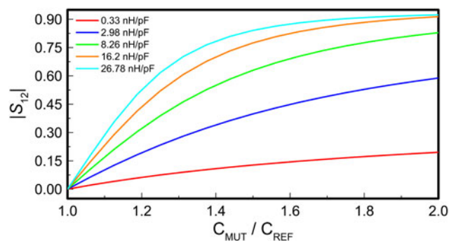
Fig. 5. Variation of |S_{12}| at f_0 = 2.894 GHz with the capacitance of the MUT as compared to the REF capacitance. REF and MUT conductance are identical and equal to 0.122 mS. Note that when C_{\text{REF}} and C_{\text{MUT}} are equal, the modulus of the cross-mode transmission coefficient is zero (perfect symmetry case).
