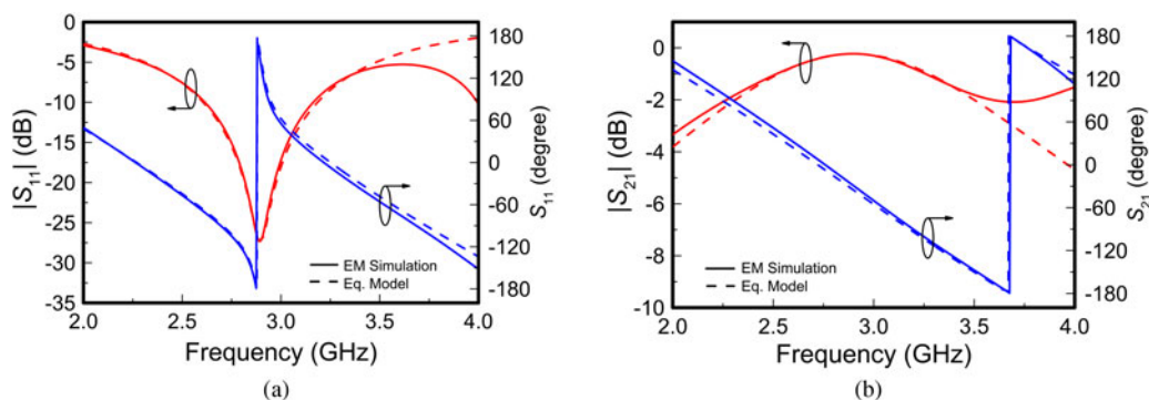
Fig. 3. Response of the OSRR of Fig. 2. (a) Reflection coefficient; (b) transmission coefficient. The extracted parameters of the bare OSRR are C_u = 0.424 pF, L = 9.228 nH, G_u = 0.124 mS, C_1 = 0.429 pF, C_2 = 0.625 pF, Z_0 = 50 \Omega and \beta l = 118.7^\circ .
