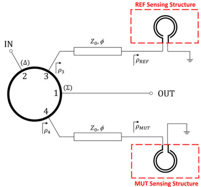
Fig. 1. Topology of the proposed reflective-mode differential sensor.
