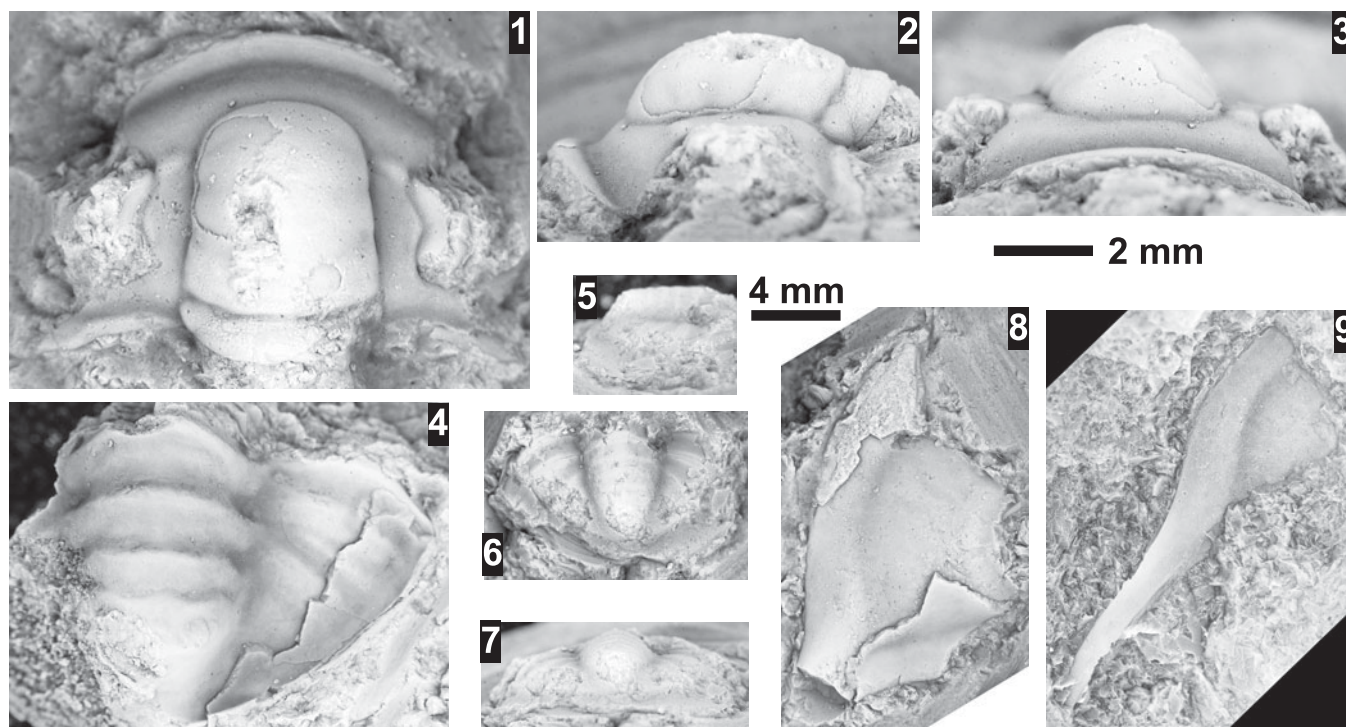
Figure 11. Trilobites from the Elvinia Biozone, Steptoean Stage, St. Charles Formation, Smithfield Canyon, Utah. All specimens are from USNM loc. 44301. (1–3) Pseudosaratogia sp. indet. partially exfoliated cranium USNM 775657: (1) dorsal view; (2) lateral view; (3) anterior view. (4) Elvinia sp. indet. mostly exfoliated pygidium USNM 775661. (5–9) Iddingsia sp. indet.: (5–7) exfoliated pygidium USNM 775658: (5) lateral view; (6) dorsal view; (7) posterior view; (8) mostly exfoliated librigena USNM 775660; (9) exfoliated librigena USNM 775659. (1–3) Specimens use the 2 mm scale bar; (4–9) specimens use the 4 mm scale bar.
