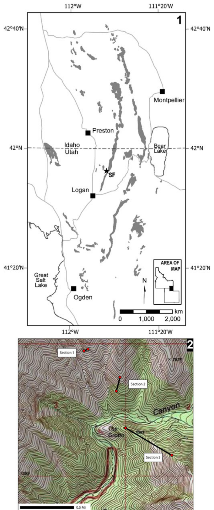
Figure 1. (1) Map showing the location of the Smithfield Canyon section (black star, “SF”) in regional context. Gray polygons represent the aerial extent of mapped Nounan and St. Charles formations. Modified from the Stage Geologic Map Compilation (Horton et al., 2017) and Wakeley (1975). (2) Portion of the Naomi Peak 7.5-foot quadrangle showing the locations of the three measured sections. Basemap: 2013 National Geographic USA topographic map, projection: NAD 1983 UTM Zone 12N.
