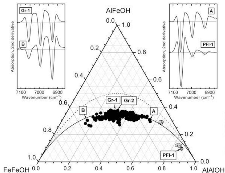
Figure 3. Occupancy of the M2M2 dioctahedral pairs of palygorskite by AlAlOH , AlFe^{III}OH and Fe^{III}Fe^{III}OH . 177 Pefkaki samples containing >20% palygorskite (black), nine commercial samples of unknown origin (light gray) and PFI-1 (dark gray) are shown. The solid arc is a guide through the experimental points and the dotted arc corresponds to the statistical distribution of Al and Fe^{III} in the M2M2 pairs. Insets show details of the 2 nd derivative spectra of characteristic samples, and define how intensities have been measured.
