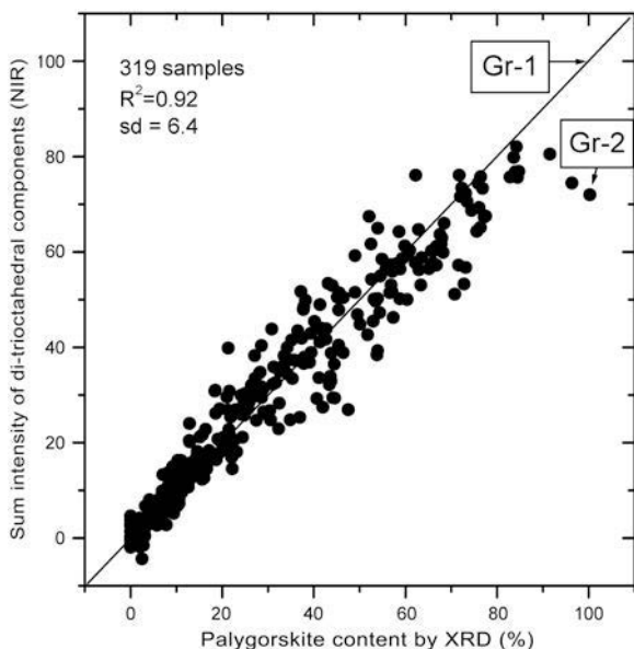
Figure 9. Correlation between the total (dioctahedral + trioctahedral) palygorskite contents of the Pefkaki samples estimated from the NIR and XRD data, and normalized to palygorskite Gr-1. For details see the text.
