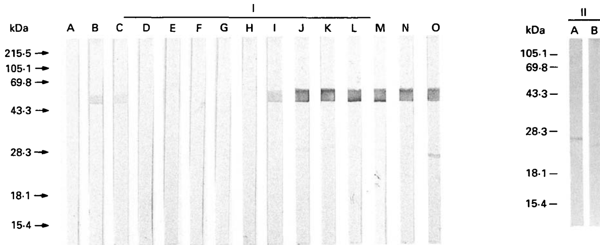
Fig. 5. II Western blot of total T. cruzi (A) and T. rangeli (B) antigens reacted with mouse immune serum to Tc24 recombinant protein.
