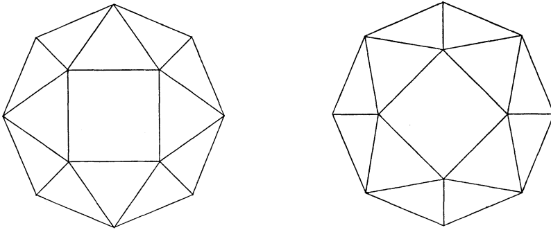
Snub square antiprism
