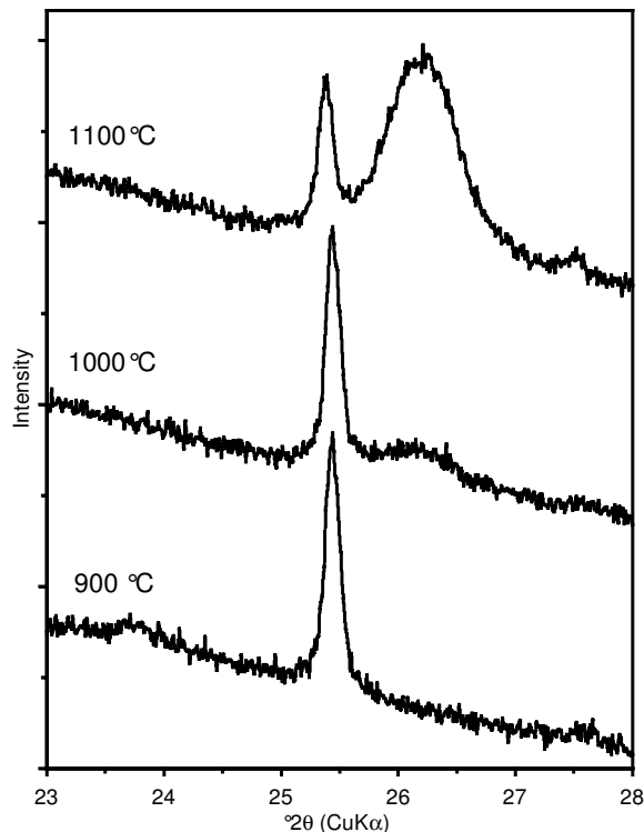
Figure 3. XRD patterns of the Amazon kaolin fired at (from bottom to top) 900, 1000 and 1100°C. Note the prominent anatase 101 peak at \sim 25.4^\circ 2\theta ( 3.50 \text{ \AA} ) and the gradual appearance of the (still unresolved) mullite 120 and 210 peaks at \sim 26.2^\circ 2\theta . The y axis scale divisions correspond to 5 counts per second.
