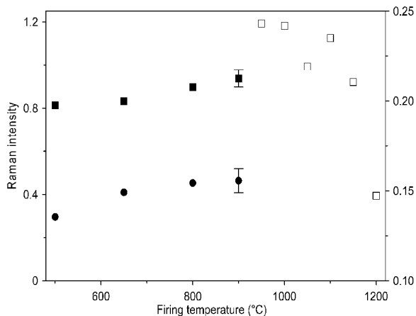
Figure 1. Intensities of the Raman E_g bands at \sim 144 (squares and left y axis) and 639\text{ cm}^{-1} (closed circles and right y axis) in the Amazon kaolin as a function of the firing temperature. The closed squares outline the field in which other anatase bands were also observed, whereas no other bands could be discerned at higher temperatures (open squares). Error bars shown for the sample fired at 900^\circ\text{C} indicate the standard deviations for the two anatase bands.
