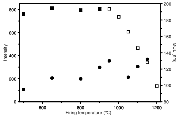
Figure 4. Intensities of the anatase 110 XRD peak at \sim 25.4^\circ 2\theta ( 3.50 \text{ \AA} ) in the Amazon kaolin (squares and left y axis) and mean coherence lengths, which are taken as a measure of particle size (circles and right y axis), as a function of the firing temperature. The closed symbols outline the field in which anatase Raman bands, besides that at \sim 144 , were also observed.
