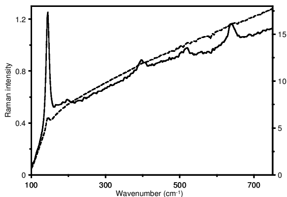
Figure 2. Raman spectra of the Amazon kaolin fired at 900^\circ\text{C} (solid line) and 950^\circ\text{C} (broken line) showing the anatase bands at 398 , 515 and 639\text{ cm}^{-1} at 900^\circ\text{C} and the unfavorable signal/background ratio at 950^\circ\text{C} . The left and right y axes refer to the samples fired at 900 and 950^\circ\text{C} , respectively.
