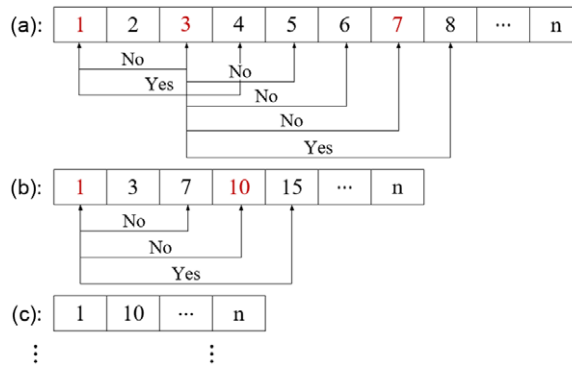
Figure 11. Node optimization of feasible paths.
