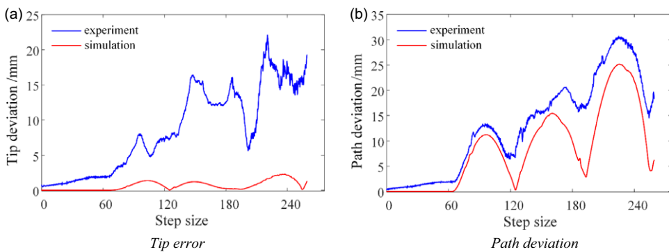
Figure 22. Error comparison between experiment and simulation at each step.
