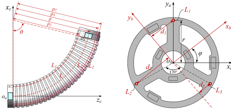
Figure 4. Kinematics of driving parameters.
