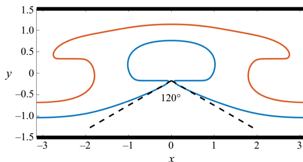
Figure 4. Almost limiting wave profile in figure 3(cii) in one spatial period. The black dashed line represents the limiting 120^\circ angle.
