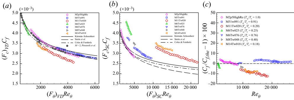
Figure 3. Transformed skin friction coefficient ( C_{f,i} = F_c C_f ) versus Reynolds numbers ( Re_{\theta,i} = F_\theta Re_\theta ) based on (a) the van Driest II theory and (b) the Spalding & Chi theory, wherein the black solid line, the dashed line and the dash-dotted line denote the incompressible correlations of Kármán–Schoenherr (Roy & Blottner 2006), Smits et al. (1983) and Coles–Fernholz (Nagib et al. 2007), respectively. The relative difference between the DNS and the theoretical prediction based on a combination of van Driest II transformation with the power-law relation of Smits et al. (1983) (i.e. C_{f,the} = (C_{f,i})_{SM} / (F_c)_{VD} ) is shown in (c).
