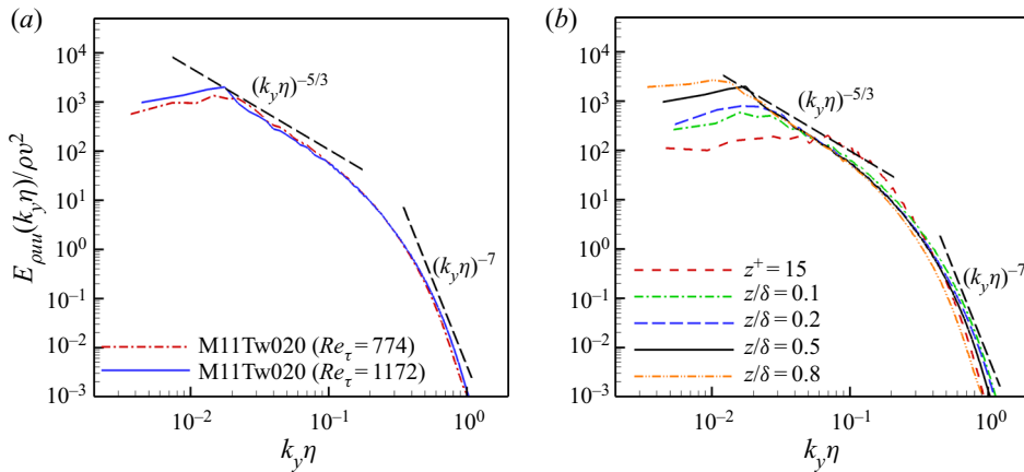
Figure 29. One-dimensional energy spectra of case M11Tw020 as a function of the spanwise wavenumber, k_y : (a) for two different Reynolds numbers at z/\delta \approx 0.5 ; and (b) at multiple heights for Re_\tau = 1172 . Here, \eta = \bar{\rho}^{-1/2}(\mu^3/\phi)^{1/4} and v = \bar{\rho}^{-1/2}(\mu\phi)^{1/4} are the Kolmogorov length and velocity scales, respectively, where \phi = \tau'_{ik}(\partial u'_i/\partial x_k) is the viscous dissipation rate per unit volume (Zhang et al. 2018).
