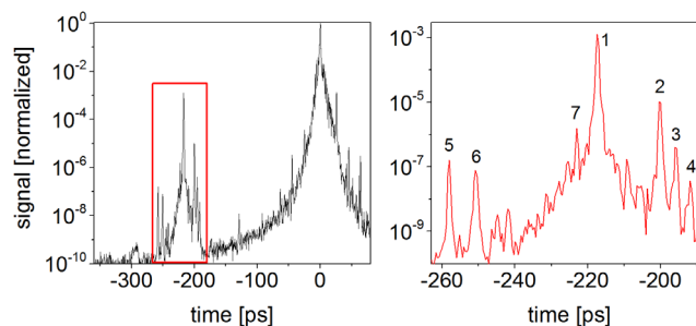
Figure 4. Temporal profile of the PHELIX pulse in 2012 using the uOPA with a gain of 10^4 . The pulse was measured with a third order cross-correlator (Sequoia, Amplitude Technologies). The right graph shows an enlargement of the red framed region of the left graph.
