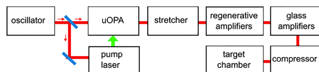
Figure 3. Schematic of the PHELIX short pulse beamline.
