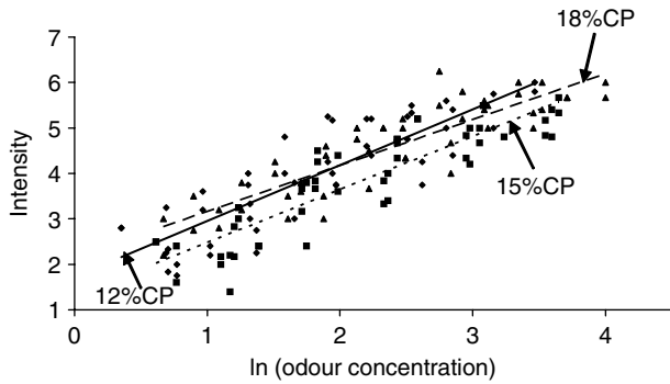
Figure 3 Odour intensity (I) as a function of odour concentration with regression lines, I_{12\%CP} = 1.95 (0.13) + 1.13 (0.05) \ln (\text{odour concentration}) , indicated by \text{---} \blacklozenge ; I_{15\%CP} = 1.40 (0.14) + 1.13 (0.05) \ln (\text{odour concentration}) , indicated by \text{.....} \blacksquare ; I_{18\%CP} = 1.83 (0.15) + 1.13 (0.05) \ln (\text{odour concentration}) , indicated by \text{---} \blacktriangle , R^2 = 77.5\% .
