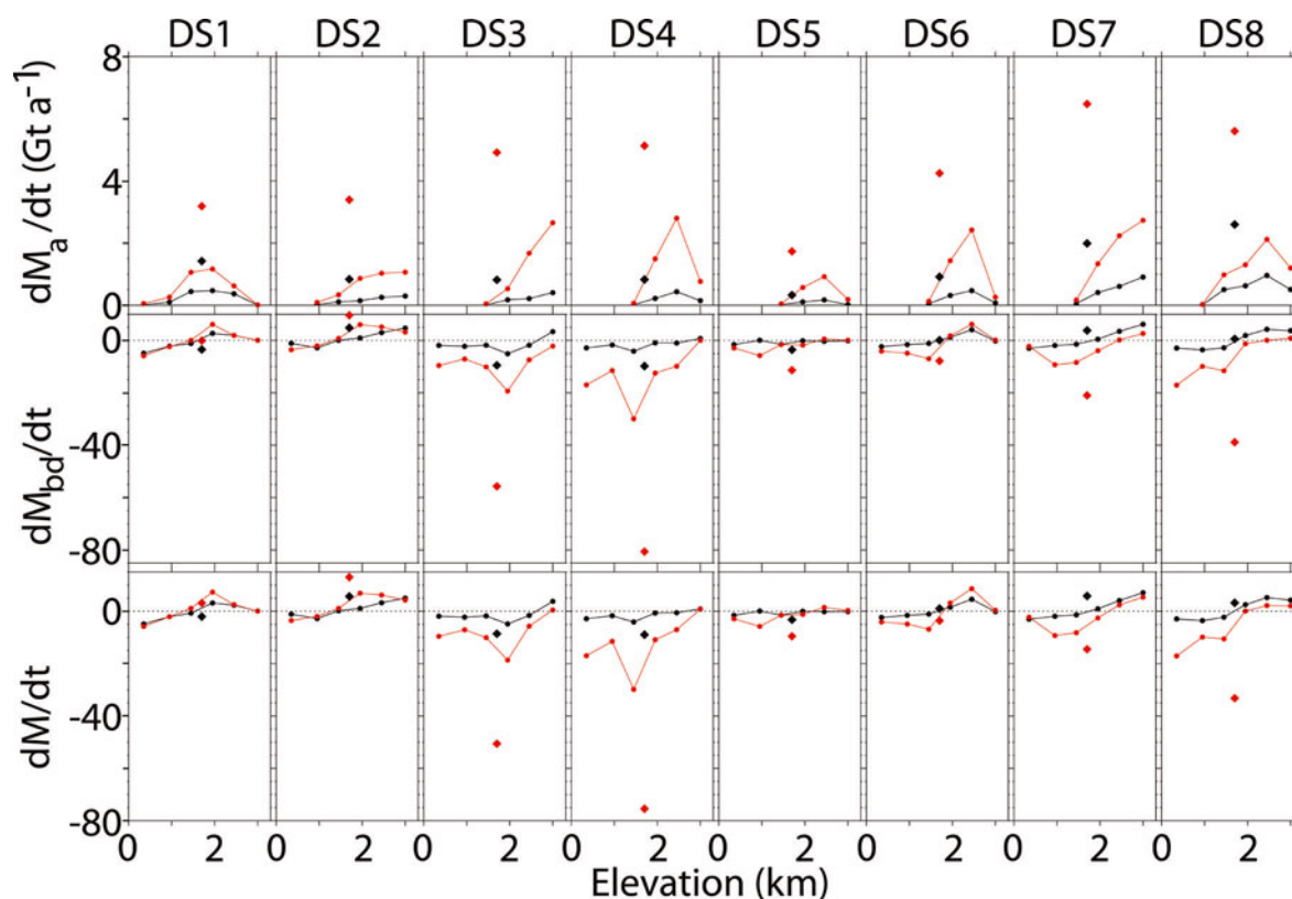
Fig. 12. Components of mass change by drainage system. dM_a/dt , dM_{b,d}/dt , dM/dt ( \text{Gt a}^{-1} ) averaged over 500 m elevation bands for the eight drainage systems for 1992–2002 (black) and 2003–07 (red) with totals for 1992–2002 (black symbols) and 2003–07 (red symbols). Accumulation-driven mass increases are largest in DS3, DS4, DS7 and DS8, and dynamic-/ablation-driven thinning is largest in DS3, DS4 and DS8 and very small in DS1, DS2, DS5 and DS6.
