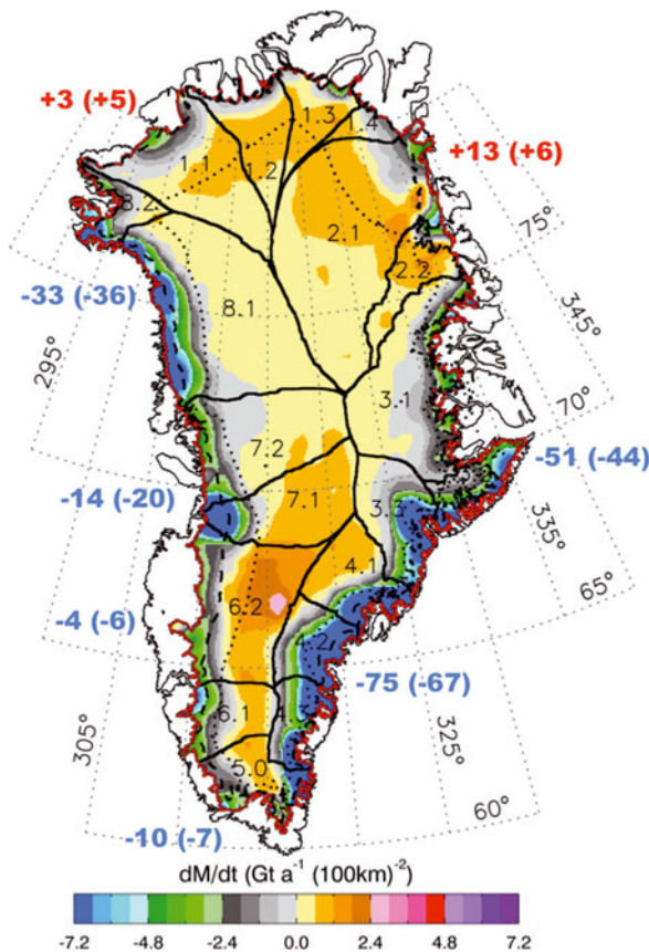
Fig. 8. Map of dM/dt ( Gt\ a^{-1}\ (100km)^{-2} ) for 2003–07 derived from ICESat data. The numbers around the map are the net gains (red) or losses (blue) ( Gt\ a^{-1} ) for the DS1–DS7. The numbers in parentheses are the changes from the 1992–2002 period. All drainage systems except DS5 are divided into subsystems (e.g. DS1.1, etc.). The largest increases in the rates of mass loss are in the west central region and the southeast. The northern DS1 and DS2 are gaining mass. Most of the areas above and below 2000 m (dotted curve) are gaining and losing mass, respectively. Mass losses below the EL (dashed curve) are from a combination of increased melting and acceleration of outlet glaciers.
