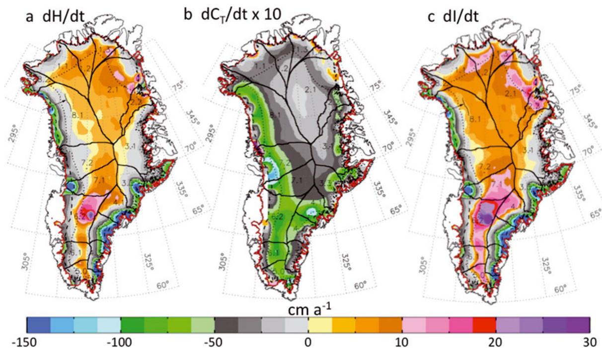
Fig. 4. (a) ICESat dH/dt = \langle dh/dt \rangle averaged in \sim 50 km gridcells. (b) Temperature-driven part of the firm compaction dC_T/dt times 10. (c) dl/dt = (dH/dt) - (dC_T/dt) - (dB/dt) . Although dC_T/dt is generally smaller than dH/dt , it shifts the dH/dt = 0 line by \sim 100 km in the northwest as shown by the arrows. In addition to the delineation of the drainage systems (black curves), the 2000 m contour (dotted curve), the EL (dashed curve) and the ice-sheet boundary (red curve) are shown here and in Figures 5–9.
