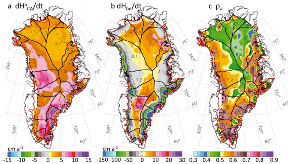
Fig. 7. Maps for the 2003–07 period. (a) Accumulation-driven elevation change, dH^a_{CA}/dt . (b) Ablation- and dynamic-driven elevation change, dH_{bd}/dt . (c) Relative density, \rho_a , of the firn for the dH^a_{CA}/dt component.
