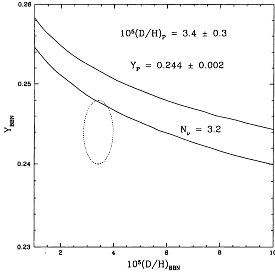
Figure 2. As Figure 1, but for N_\nu = 3.2
