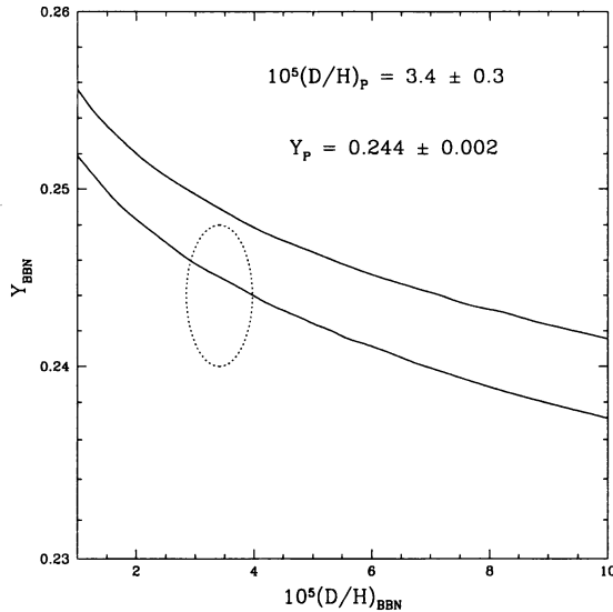
Figure 1. The SBBN-predicted {}^4\text{He} mass fraction Y_P as a function of the SBBN-predicted primordial deuterium-to-hydrogen ratio D/H is shown (at the \pm 2\sigma level) by the solid lines. The dotted ellipse is the 95% contour of the BT deuterium abundance and the IT {}^4\text{He} mass fraction (see the text).
