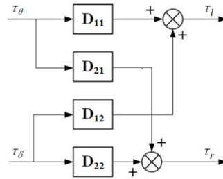
Fig. 6. State-space model decoupling process.
