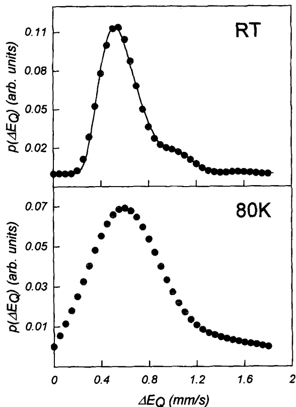
Figure 2. Quadrupole-splitting distribution profiles p(\Delta E_Q) of the LS07 Al-lepidocrocite at room temperature and 80 K. The size of the symbols corresponds to the step (0.05 mm/s) at which the quadrupole splitting was allowed to vary within the range 0.0–1.8 mm/s. The full line in (RT) represents the superposition of two log-normal distributions adjusted to the calculated probability values.
