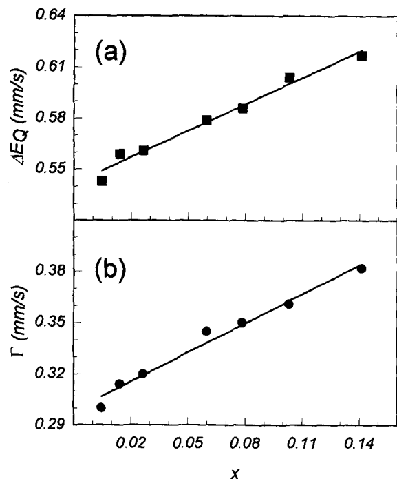
Figure 1. Quadrupole splitting \Delta E_Q (a) and line width \Gamma (b) for the lepidocrocite samples at room temperature plotted as a function of the Al content x in \gamma\text{-Fe}_{1-x}\text{Al}_x\text{OOH} . The Mössbauer spectra were fitted with a symmetrical quadrupole doublet. The solid lines are the linear-regression lines.
