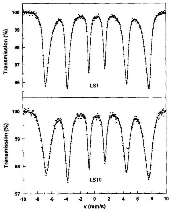
Figure 5. Mössbauer spectra at 8 K of the Al-lepidocrocite samples LS1 and LS10. The full curves are the adjusted spectra calculated with a model-independent distribution of hyperfine fields.
