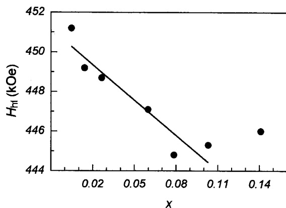
Figure 6. Maximum-probability hyperfine field H_{\text{hf}}^{\text{m}} derived from the 8 K Mössbauer spectra plotted as a function of the Al content x . Solid curve is the linear-regression line for data of samples LS02 to LS10.
