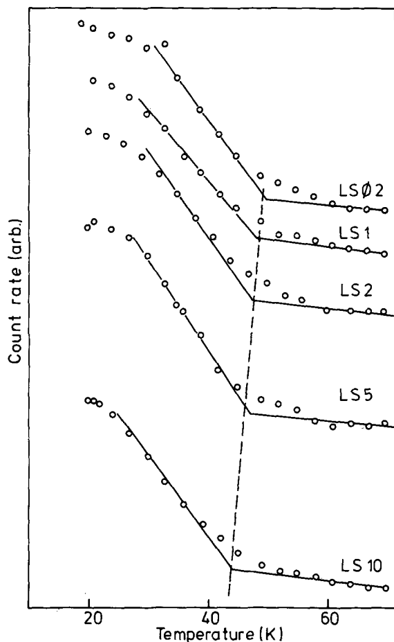
Figure 3. Thermo-scan curves measured for 5 of the 7 investigated lepidocrocite samples. The dashed line shows the slight decrease with increasing initial Al contents C_i of the temperature at which the onset of magnetic ordering is detected.
