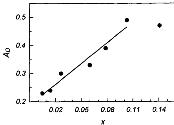
Figure 4. Fractional doublet area A_D in the mixed Mössbauer spectra recorded at 35 K plotted as a function of the Al content x . Solid curve serves as a guide for the eye.
