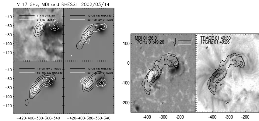
Figure 1. RHESSI and Nobeyama maps showing the multi-loop configuration of the 2002 March 14 flare. Left panel: A sequence of 12-25 keV RHESSI maps overlain on MDI (top left) and 17 GHz V images. Right panel: The remote source (upper right) seen at 17 GHz but not in HXR, and its connection to the main source (lower left) in 17 GHz maps. These are overlain on MDI (left) and TRACE (right) images.
