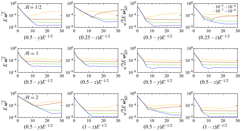
Figure 7. Profiles of scaled \overline{\omega^2} and \overline{\omega_{SD}^2} in the boundary layer along the line segments shown in figure 3, (x, y, z) = (0, y, 0) and (x, y, z) = (0, 0, z) , for \mathcal{R} and E = Ro as indicated.
