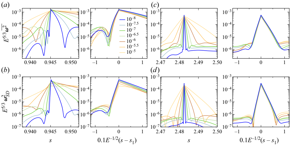
Figure 6. Rescaled profiles of \overline{\omega^2} and \omega_{SD}^2 from figure 5, showing (a,b) zoom-ins around s = s_1 = (\sqrt{1 - \omega^2} - 0.75\omega)\sqrt{5} \approx 0.9451 together with the same zoom-ins in terms of a scaled arc length centred at s_1 , and (c,d) zoom-ins around s = s_2 = (\sqrt{1 - \omega^2} + 0.5\omega)\sqrt{5} \approx 2.4824 together with the same zoom-ins in terms of a scaled arc length centred at s_2 , showing self-similarity of the peaks associated with the reflections on the short and long walls, respectively. The total length of the attractor path is L = 2s_2 \approx 4.9648 (Welfert et al. 2023, (2.34)).
