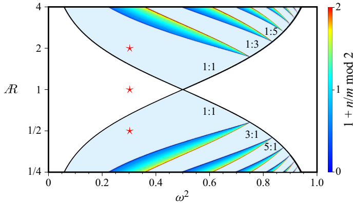
Figure 2. Inviscid (\omega^2, \mathcal{R}) -regime diagram for wave beams in the plane x = 0 : the bold black curves \omega^2 = 1/(1 + \mathcal{R}^{\pm 2}) delimit regions of differing criticality of wave beam reflections on the walls at y = \pm 0.5 or z = \pm 0.5\mathcal{R} and focusing of the beams onto m : n or n : m attractors. The red stars correspond to cases discussed in this study. The figure has been adapted from Welfert et al. (2023).
