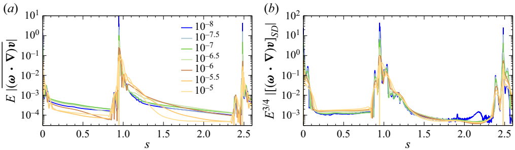
Figure 13. Scaled |\overline{(\boldsymbol{\omega} \cdot \nabla)\mathbf{v}}| and |[(\boldsymbol{\omega} \cdot \nabla)\mathbf{v}]_{SD}| as functions of arc length s along the attractor (localised using VEBA), for \mathcal{R} = 2 and E = Ro as indicated.
