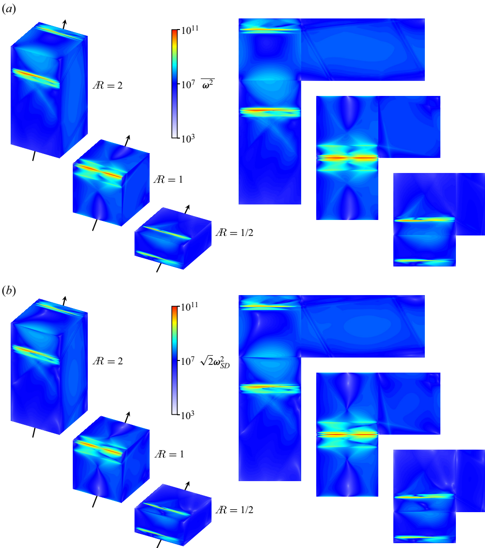
Figure 9. Perspective and unfolded views of (a) \overline{\omega^2} and (b) \sqrt{2}\omega_{SD}^2 on the cuboid surfaces for E = Ro = 10^{-8} and \mathcal{R} as indicated. Supplementary movie 2 animates \omega^2 on the surface over a libration period \tau = \pi/\omega .
