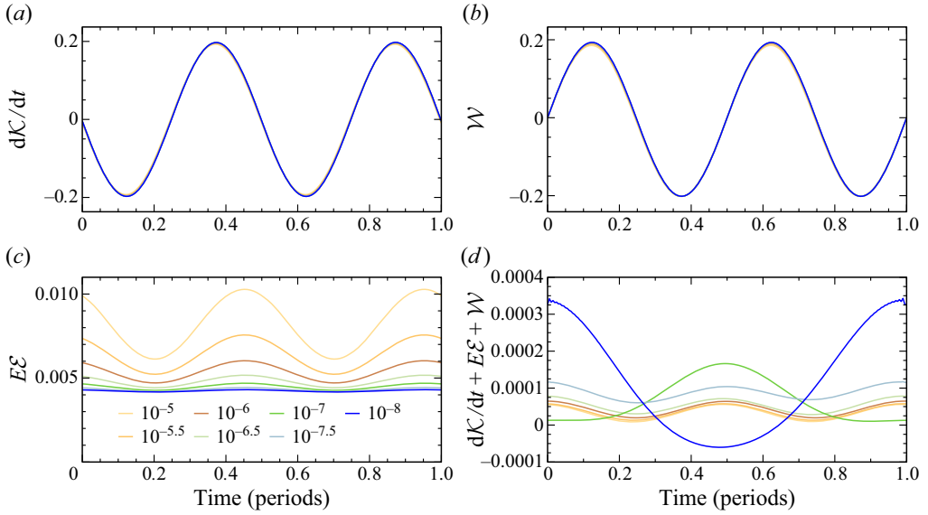
Figure 16. Variations over one libration period of the three terms on the left-hand side of (5.5), d\mathcal{K}/dt , E\mathcal{E} and \mathcal{W}(\mathbf{v}) , and their sum, for \mathcal{R} = 2 and E = Ro as indicated.
