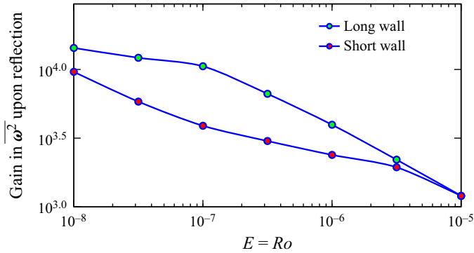
Figure 11. Gains in \overline{\omega^2} at reflections at x = 0 on the long and short walls as functions of E and Ro for \mathcal{R} = 2 .
