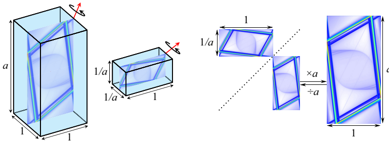
Figure 18. Relationship between flows in 1 \times 1 \times a and 1/a \times 1 \times 1/a cuboids.
