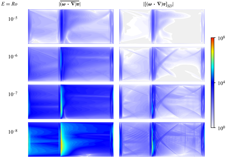
Figure 12. Illustrations of |\overline{(\boldsymbol{\omega} \cdot \nabla)\mathbf{v}}| and |[(\boldsymbol{\omega} \cdot \nabla)\mathbf{v}]_{SD}| on two branches of the attractor (the other two are the \mathcal{C} conjugates), for \mathcal{R} = 2 and E = Ro as indicated. Supplementary movie 3 includes animations of |(\boldsymbol{\omega} \cdot \nabla)\mathbf{v}| over one libration period.
