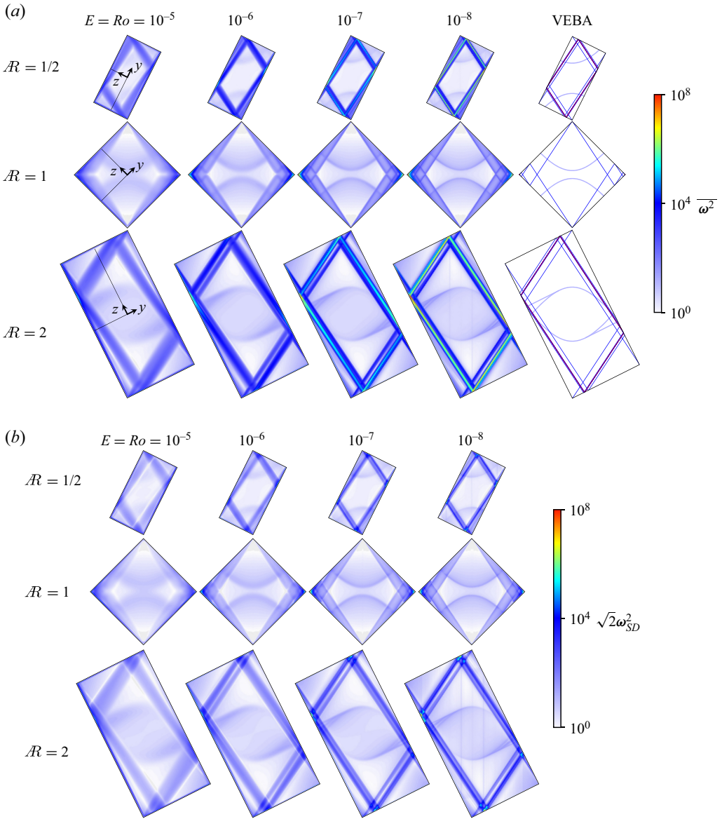
Figure 3. (a) Mean enstrophy density \overline{\omega^2} and (b) standard deviation of the enstrophy density \sqrt{2}\omega_{SD}^2 in the meridional plane x = 0 (where the rotation axis is vertical through the top and bottom corners), for \mathcal{R} and E = Ro as indicated. The last column in (a) has the VEBA results showing beams emitted from the four corners in blue and the attractor in red; traces of the primary conic beams emitted from the vertices of the cuboid and planar beams emitted from edges at x = \pm 0.5 are in light blue. Secondary traces due to reflections of these beams, which are visible in the DNS, are not included in VEBA. The black lines through the origin in panels in the first column of (a), (0, y, 0) and (0, 0, z) , are used to plot profiles of \overline{\omega^2} and \omega_{SD}^2 in figure 4. Supplementary movie 1 (available at https://doi.org/10.1017/jfm.2023.772 ) animates \omega^2 for the E = Ro = 10^{-8} cases over one libration period \tau = \pi/\omega .
