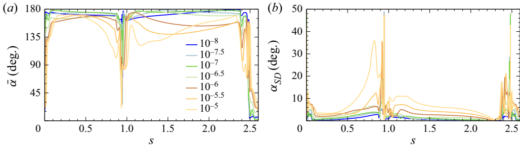
Figure 14. Variations of the mean and standard deviation of \alpha = \arccos(\hat{v} \cdot \hat{\omega}) with arc length s along the attractor (localised using VEBA) at x = 0 , for \mathcal{R} = 2 and E = Ro as indicated. Only two branches of the attractor are shown; on the other two branches, the mean angle is 180^\circ - \bar{\alpha} and the standard deviation is the same.
