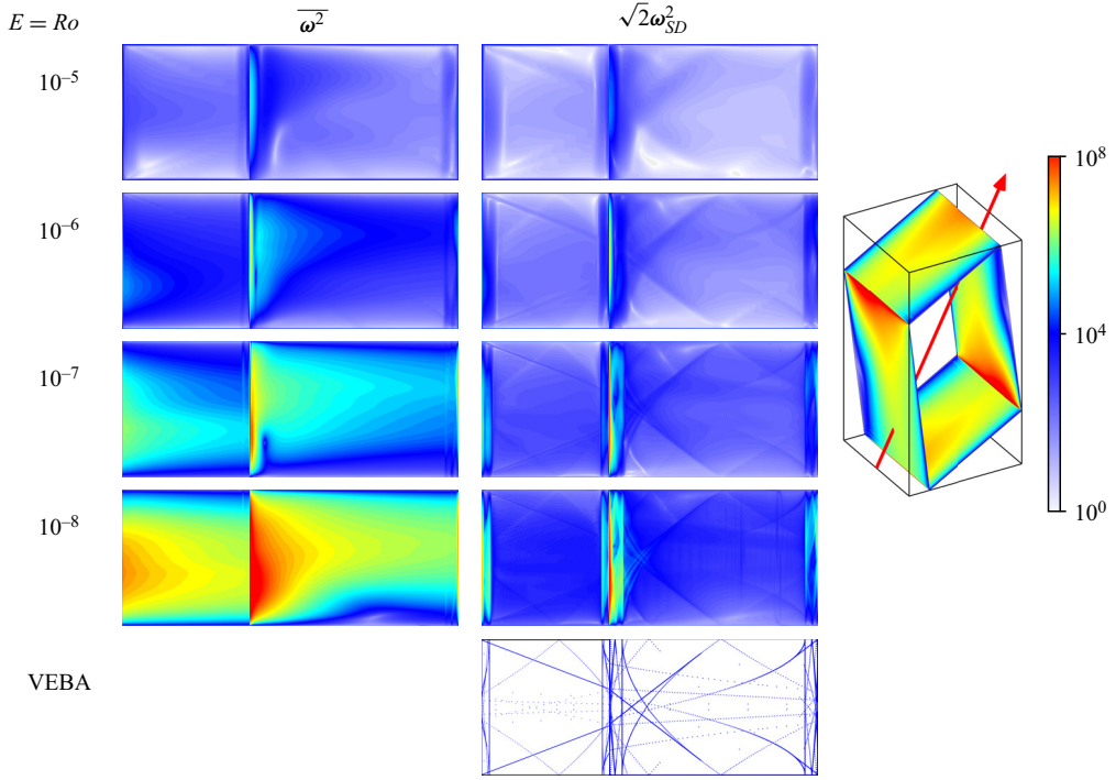
Figure 10. Illustrations of \overline{\omega^2} and \sqrt{2}\omega_{SD}^2 on two branches of the attractor (the other two are the \mathcal{C} conjugates), for \mathcal{R} = 2 and E = Ro as indicated, as well as a 3-D perspective of \overline{\omega^2} on the attractor for the case E = 10^{-8} . The bottom row presents intersections with the attractor of the wave beams emitted from edges and vertices, and their subsequent reflections, as determined via VEBA. Supplementary movie 3 includes animations of \omega^2 over one libration period.
