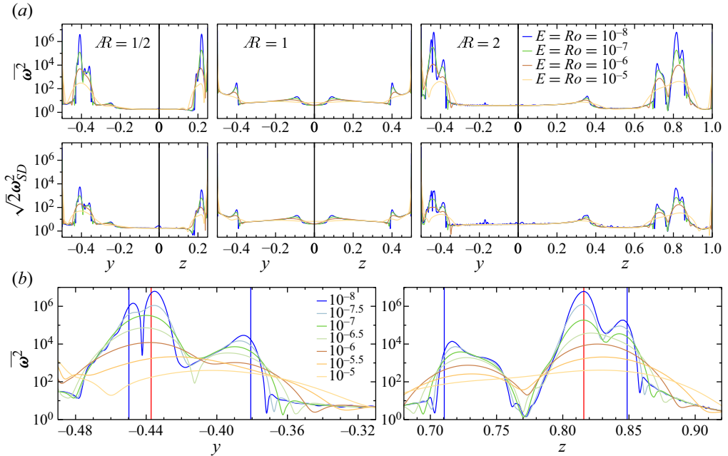
Figure 4. (a) Profiles of \bar{\omega}^2 and \sqrt{2}\omega_{SD}^2 along the line segments shown in figure 3, (x, y, z) = (0, y, 0) and (x, y, z) = (0, 0, z) , for \mathcal{R} and E = Ro as indicated. (b) Zoom-ins for the \mathcal{R} = 2 cases in the attractor regions, with additional intermediate values of E and Ro as indicated. The vertical lines correspond to the locations as determined by VEBA of the attractor (in red) and primary (before any reflection, farther away from the red line) or secondary (after one wall reflection, closer to the red line) vortex sheets originating from tropical or polar edges (in blue); compare with the VEBA panel from figure 3(a). Note the more rapid growth of \bar{\omega}^2 at the attractor.
