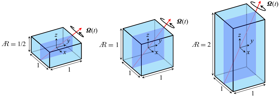
Figure 1. Schematic of the cuboid librating around its axis of rotation \boldsymbol{\Omega}(t) , for aspect ratios \mathcal{R} as indicated; the meridional plane x = 0 is shown in blue.
