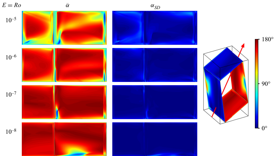
Figure 15. Mean and standard deviation of the angle between velocity and vorticity, \alpha = \arccos(\hat{\omega} \cdot \hat{v}) , on two branches of the attractor, for \mathcal{R} = 2 and E = Ro as indicated, as well as a 3-D perspective of \bar{\alpha} on the attractor for the case E = 10^{-8} . Supplementary movie 3 includes animations of \alpha over one libration period.
