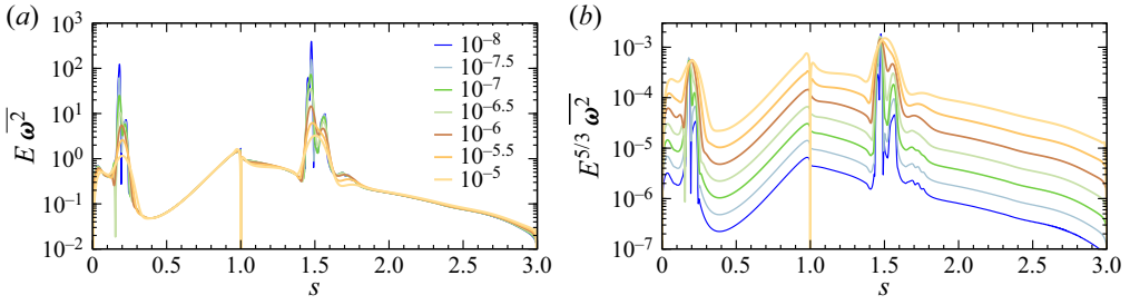
Figure 8. Scaled \overline{\omega^2} along the boundary at x = 0 , for \mathcal{R} = 2 and E = Ro as indicated.
