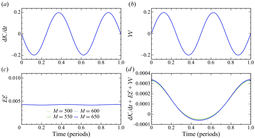
Figure 17. Variations over one libration period of the three terms on the left-hand side of (5.5), dK/dt , E\mathcal{E} and \mathcal{W}(\mathbf{v}) , and their sum, for \mathcal{R} = 2 and E = Ro = 10^{-8} , and spatial resolution M as indicated.
