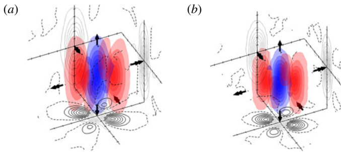
FIGURE 1. Conditional Q field for a strain-dominated region in the eigenframe of the strain tensor. (a) DNS data and (b) experimental data. Figures from Lawson & Dawson (2015), reused with permission of the authors.
