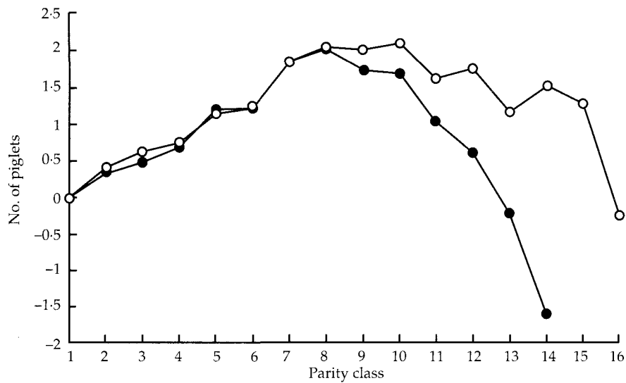
Figure 1 Parity class effects (expressed as deviations from parity class 1) on number of piglets born in Danish Landrace (●) and Yorkshire (○); first parity is divided into five classes according to age of gilt at farrowing.
