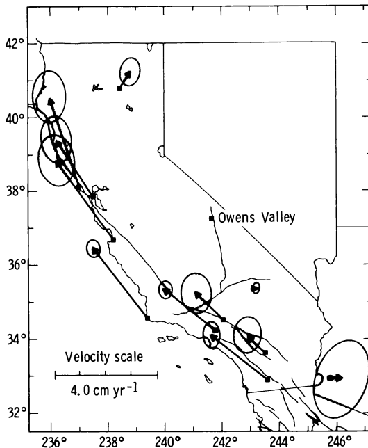
Figure 1. Velocities of VLBI sites relative to the site at the Owens Valley Radio Observatory which is assumed fixed. Error ellipses represent one standard deviation.
