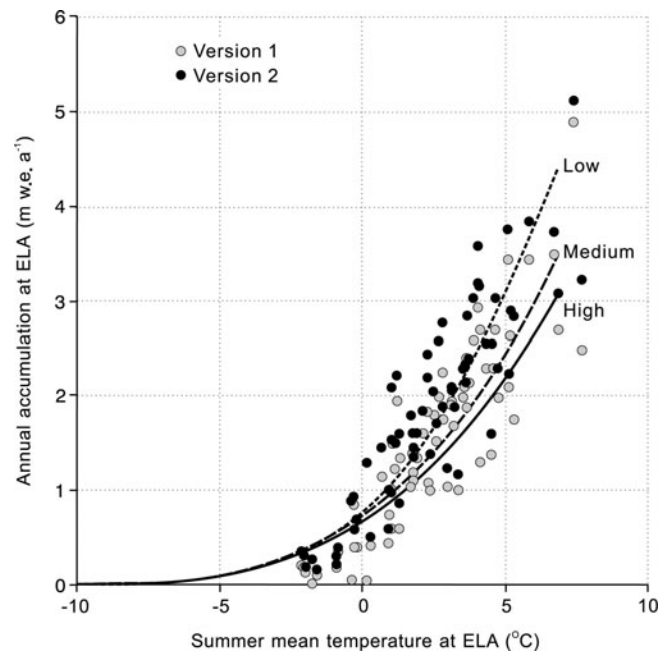
Fig. 5. Annual accumulation at the ELA plotted against summer (June–August) mean temperature ( T_{6-8} ) for 66 glaciers from Ohmura and others (1992). Version 1 refers to winter balance, and version 2 refers to 'winter balance plus summer precipitation'. Curves are for the degree-day model with 'low', 'medium' and 'high' values of annual temperature range, respectively 15, 25 and 35 K.
