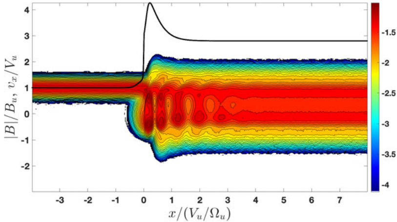
FIGURE 6. The reduced distribution function f(x, v_x) = \int f(x, \mathbf{v}) dv_y dv_z obtained by tracing 80 000 ions through the structured shock profile. The black line shows the magnetic field magnitude.
