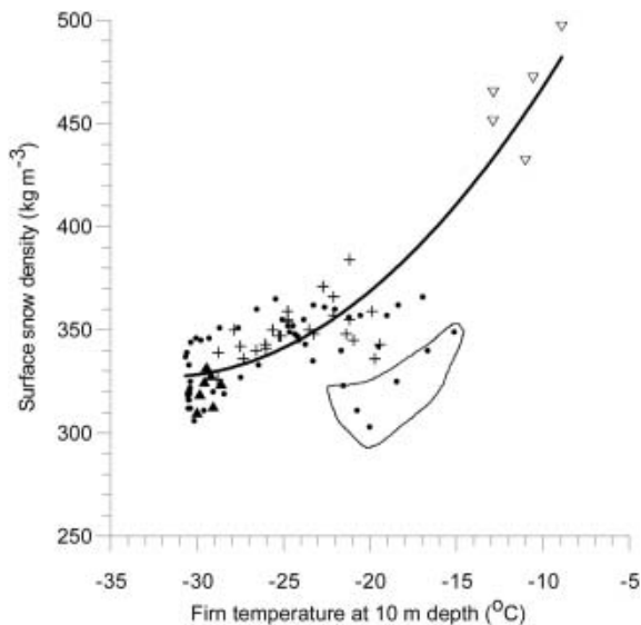
Fig. 2. Surface snow density on the Greenland ice sheet vs 10 m firn temperature. Data sources: filled circles: Benson (1962); open triangles: Braithwaite and others (1994); crosses: Mosley-Thompson and others (2001); filled triangles: H.B. Clausen (personal communication, 2004). Full curve represents a least-squares quadratic fit. Points within the thin closed curve are omitted from the fitting procedure (see text for explanation).
