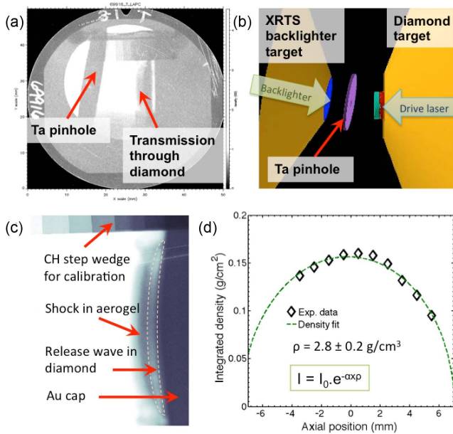
Figure 7. An example of X-ray radiographic measurement on warm dense carbon carried out by Falk et al. [52, 142] . A diamond sample was driven by laser with 5 \times 10^{14} W/cm 2 intensity. A point projection radiography setup with 30 \mu m pinhole and Vanadium He- \alpha backlighter at 5.2 keV were used. (a) An example of the X-ray film used for the radiographic measurement, (b) model of the target layout including the Ni He- \alpha backlighter and pinhole used for XRTS measurement as viewed by the radiography film, (c) detail of the radiographic measurement including the CH step wedge used for X-ray intensity calibration, and (d) Abel inversion plot used to extract the density from shock-released diamond.
