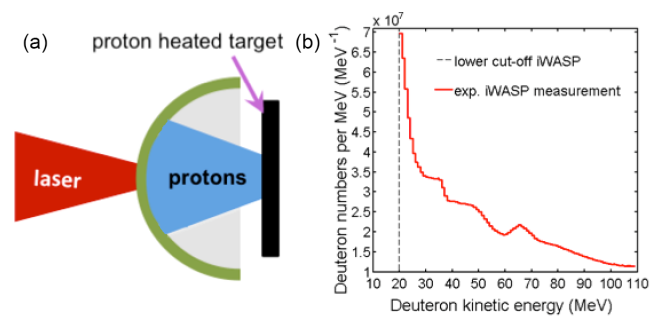
Figure 4. Laser-ion acceleration for isochoric heating: (a) a curved target for focusing of ion beams for isochoric heating to generate WDM as used by Patel et al. [54] , (b) a typical deuteron BOA spectrum taken at the Trident laser facility obtained by the iWASP diagnostic [123] .
