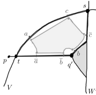
FIGURE 11. The triangle \Delta(stq') contains a central periphery Y , whose overlap with \text{Sat}_J(W') is approximated by d(b, \bar{c}) .
