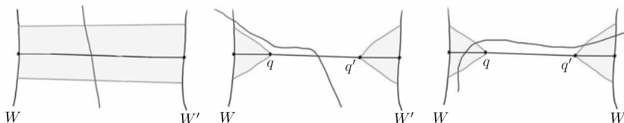
FIGURE 12. In each case, there exists W'' separating W, W' .
