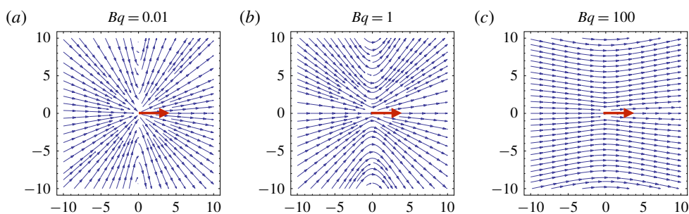
FIGURE 14. Streamlines of surface velocity as a result of a point force applied at the origin, following (3.108). Length is in units of R such that Bq = \eta_s/\eta R .
