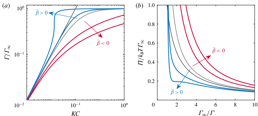
FIGURE 5. The (a) \Gamma(C) and (b) \Pi(\Gamma) relations corresponding to Frumkin adsorption from an ideal subphase. Intermolecular interactions are attractive when \tilde{\beta} = \beta\Gamma_\infty/k_B T > 0 (blue lines), and repulsive when \tilde{\beta} < 0 (red lines). Here \tilde{\beta} = 0 (grey solid lines) recovers Langmuir adsorption. The black line in each panel is the 2-D ideal gas limit (the Henry isotherm).
