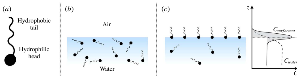
FIGURE 3. (a) Schematic representation of an amphiphilic molecule. (b,c) Surfactant molecules adsorb to the interface to an extent determined by the competition between (loss of) entropy and energetically favourable interactions during adsorption. Also shown in (c) are the concentration profiles of surfactant (solid line) and water (dashed line) molecules. The ‘excess’ surface concentration is in grey, which represents the amount of surfactant in excess of a hypothetical state where the concentration of dissolved surfactant is constant up until the surface.
