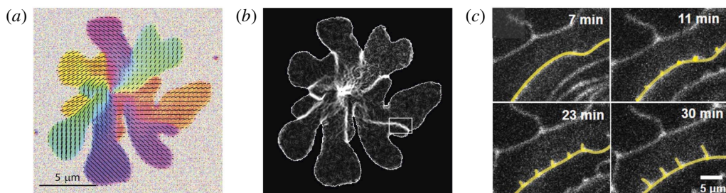
FIGURE 26. (a) Tilted DPPC tail groups within an LC domain form discrete patches, within which tails are oriented in the same direction. The tilt orientation jumps by 60^\circ from patch to patch, to accommodate the frustration between the tendency of tilt orientation to precess and the tendency of the hexagonal headgroup lattice to maintain its order. (b) Bright lines indicate boundaries between patches of aligned tilt, across which tailgroup orientation abruptly changes. These high-energy lines exert a line tension internal to the drop, effectively ‘pulling’ in invaginations at the domain boundary. (a,b) Reproduced from Dreier, Brewer & Simonsen (2012). (c) New tilt grain boundary lines form and grow in LC DPPC domain arms that had been stretched significantly. From Kim et al. (2018).
