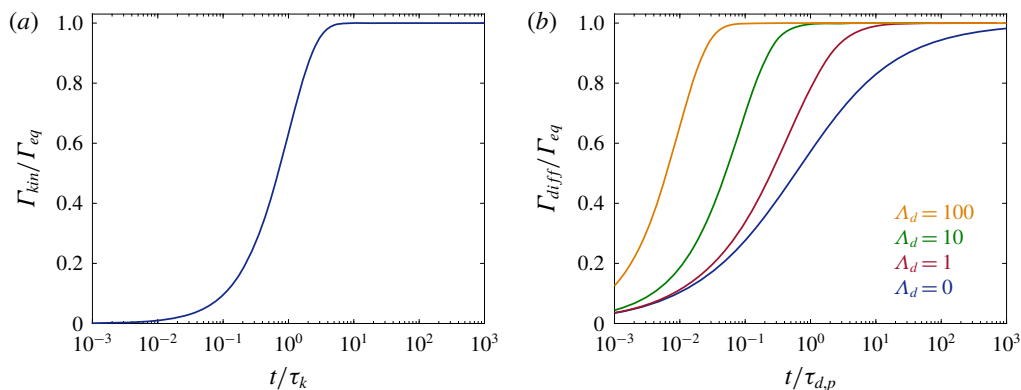
FIGURE 9. (a) Kinetically controlled adsorption (3.68) to an initially clean spherical surface. (b) Diffusion-controlled adsorption (3.71) to a spherical surface. Adsorption occurs over a faster time scale \tau_{d,s} in smaller bubbles ( \Lambda_d = L_d/R \gtrsim 1 ), and approaches equilibrium exponentially, rather than as 1/\sqrt{t} in the case of large bubbles ( \Lambda_d \rightarrow 0 ).
