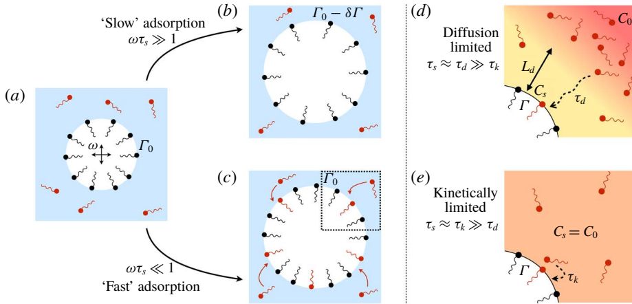
FIGURE 7. (a) A surfactant-covered bubble oscillating in a liquid containing dissolved surfactant. (b) If surfactant exchange is negligibly slow, the number of adsorbed molecules is unchanged (or the surface concentration changes by \delta\Gamma ). (c) By contrast, rapid surfactant exchange equilibrates the surface so that \Gamma(t) \approx \Gamma_0 and \delta\Gamma \approx 0 . Surfactant exchange can be (d) diffusion controlled or (e) kinetically controlled if either process is rate limiting.
