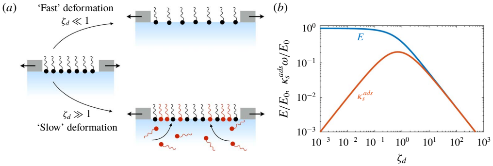
FIGURE 16. (a) Response of a surfactant monolayer to a dilatational deformation that is fast or slow relative to rate of replenishment by adsorption from the bulk. The monolayer is effectively insoluble as \zeta_d \rightarrow 0 , and the elastic modulus is highest ( =E_0 ) in this limit. Conversely, perturbations of surface concentration from equilibrium are rapidly eliminated by adsorption and the surface elasticity is weak when \zeta_d \gg 1 . (b) The dynamic Gibbs modulus E and apparent dilatational surface viscosity \kappa_s^{ads} from (4.34).
