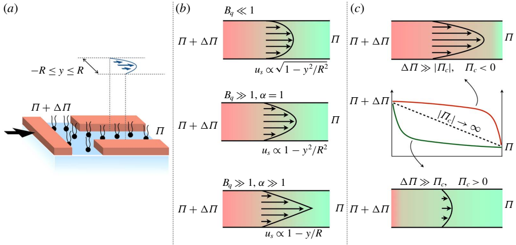
FIGURE 29. (a) A surface pressure gradient across an interfacial channel sets up a surface (and bulk) flow, much pressure-driven flow in three dimensions. (b) Illustrations of surface velocity profiles, with \alpha defined in (5.19): u_s(y) is elliptic when subphase dominant ( Bq \ll 1 ) and parabolic when interface dominant ( Bq \gg 1 ) with Newtonian surface rheology. However, condensed arachidic acid above \Pi \sim 20 \text{ mN m}^{-1} surface shear thickens, resulting in triangular velocity profiles (5.19). The background colour gradient represents \Pi(x) , which changes linearly across the length of the channel. (c) Surface pressure distribution in the channel is nonlinear when \eta_s is a function of \Pi . When \Pi -thinning, surface pressure remains of the order of the driving pressure \Delta\Pi for the majority of the channel and thus pumps a larger surfactant flux, effectively increasing the permeability of the channel. By contrast, surface pressure drops rapidly at the channel entrance when \Pi -thickening, which maintains a relatively small gradient across the rest of the channel, thereby ‘choking’ the surface flow.
