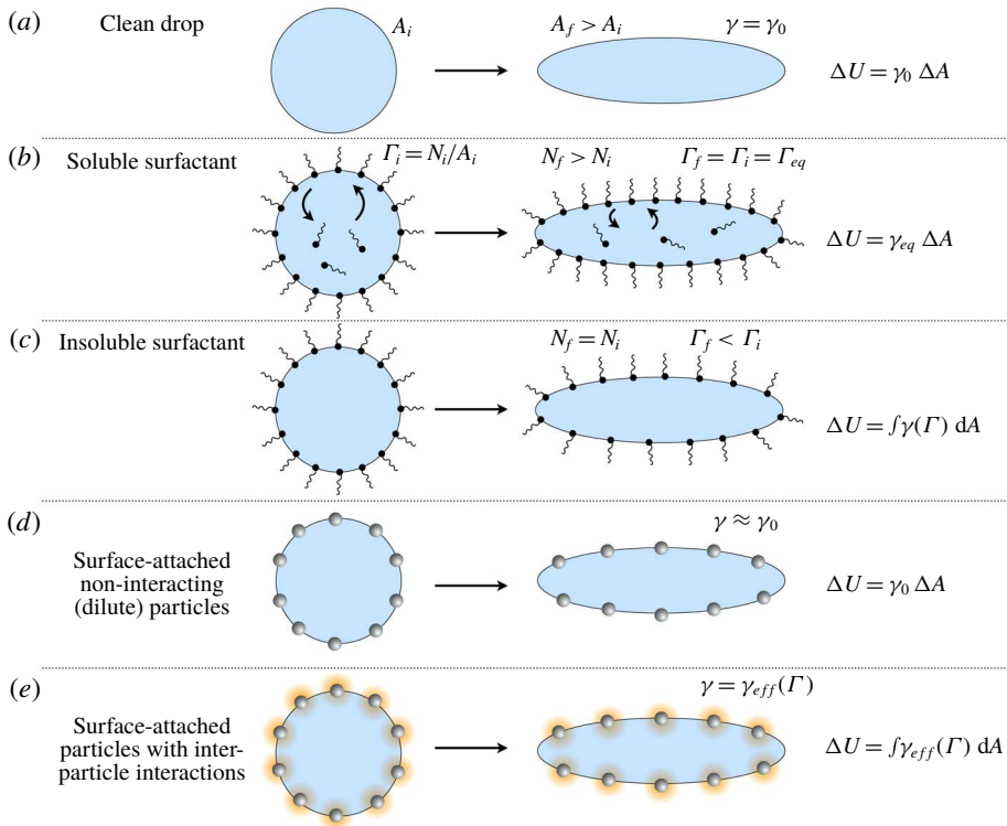
FIGURE 4. Examples of change in surface energy upon deformation of a drop with surface-active molecules or particles.
