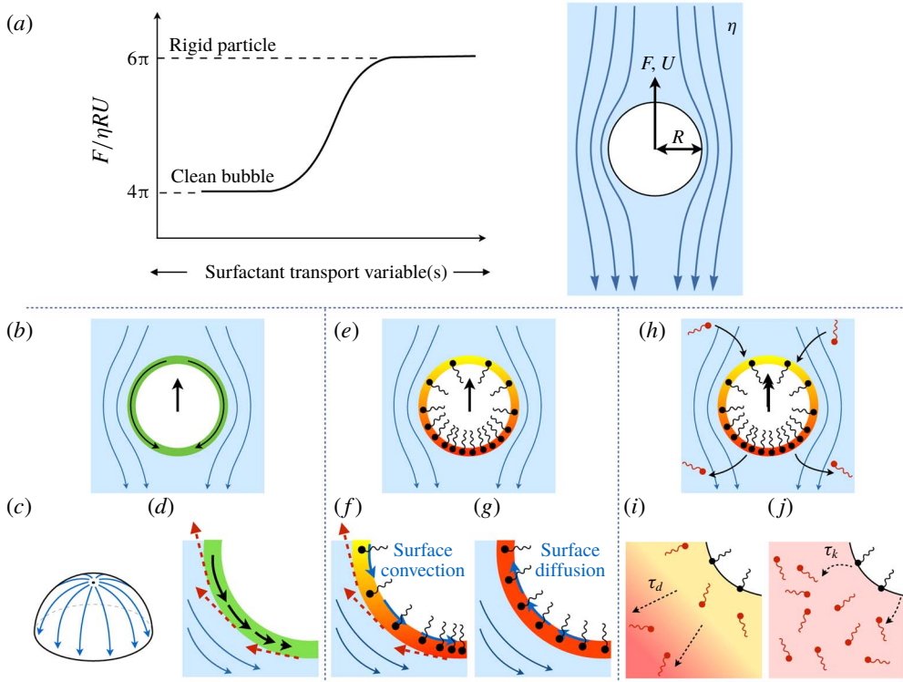
FIGURE 1. (a) ‘Hidden’ surfactant variables modify the interfacial flow of a rising bubble such that it might behave like a clean drop, a rigid particle or somewhere in between. The associated surfactant transport processes are not often easy to differentiate, and systems may exhibit one or a non-trivial combination of several processes. (b–d) For instance, an interfacial or surface excess viscosity can resist the surface flow. The solid lines depict surface flow, and dashed red arrows indicate tangential (viscous) stresses resisting deformation. (e–g) Alternatively, surfactants swept to the rear of the bubble build a concentration gradient and generate a counter-acting Marangoni stress (dashed red arrows) that resists surface convection (blue arrows). These Marangoni forces may be weakened by surface diffusion against the gradient. (h–j) If the surfactant is soluble, adsorption/desorption from the bulk can drive the surface concentration back to equilibrium over a finite time. This process might be controlled by (i) diffusive transport in the bulk across bulk concentration gradients over a time scale \tau_d , or by (j) the finite-rate kinetics over a finite time scale \tau_k .
