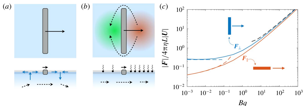
FIGURE 24. (a) A rod translating perpendicular to its long axis on a clean interface, shown in top and side views. The surface velocity field has a non-zero divergence ahead and behind the rod, and the bulk velocity field is three-dimensional. (b) Insoluble surfactants drive reverse Marangoni flows that render monolayers incompressible (see § 3.3.2 and figure 11), setting up surface and bulk flows on length scales comparable to the rod length. Surface incompressibility thus imparts a larger drag than a clean interface even when the surfactant is surface inviscid ( Bq \rightarrow 0 ), and impacts F_{\perp} more strongly than F_{\parallel} . (c) Translational resistance coefficient of long rods in incompressible monolayers (Levine et al. 2004) with asymptotic scalings in dashed lines following (4.168), (4.169) and (4.170).
