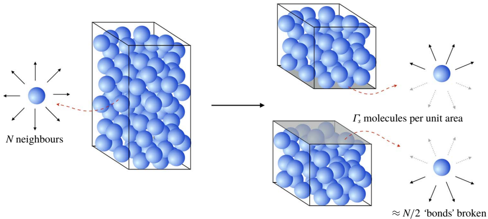
FIGURE 2. A liquid molecule in the bulk of a fluid experiences no net force due to a (time-averaged) symmetric distribution of neighbours. Creating an interface, however, requires breaking intermolecular ‘bonds’ on the interface and is energetically expensive.
