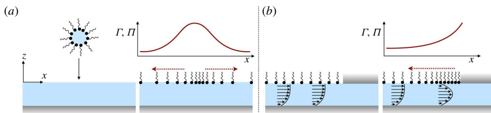
FIGURE 10. Two conjugate effects commonly termed ‘Marangoni’ effects: (a) A local increase in surfactant concentration, shown here by the addition of a surfactant-rich drop, establishes a surface concentration gradient (and, therefore, a surface pressure gradient) that drives an outward surface flow (red arrows). (b) Surface compression due to flow (in this case, towards an interfacial barrier) establishes a surface tension gradient due to non-uniform surface concentration. This introduces a reverse Marangoni flow that ‘immobilizes’ the surface.
