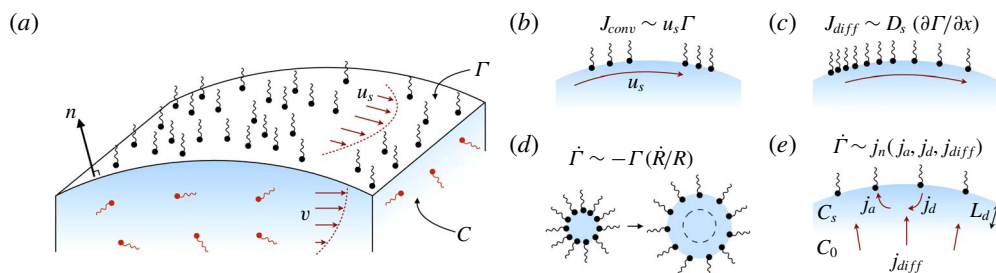
FIGURE 6. (a) Geometry of a typical surfactant-laden interface. (b–e) Mass transport processes on the interface: (b) convection due to imposed (or Marangoni) velocity u_s ; (c) diffusion due to a surface concentration gradient; (d) surface concentration evolution due to curvature modification; and (e) adsorption/desorption from the sublayer, showing the depletion length L_d .
