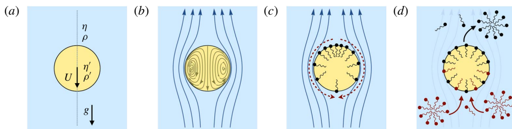
FIGURE 15. (a) A drop settling in a viscous fluid with terminal velocity U , and (b) streamlines corresponding to the Hadamard–Rybczynski solution for a clean interface. (c) The uniform retardation regime: with adsorption–desorption or diffusion over finite time scales, a surface concentration gradient is established and a reverse Marangoni flow immobilizes the surface. (d) The remobilization regime: molecules freely desorb at the downstream pole and adsorb at the upstream pole if \tau_s is small and bulk concentration is above CMC. The resulting near-uniform surface concentration suppresses Marangoni flows and remobilizes the interface.
