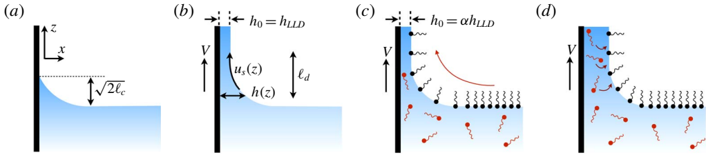
FIGURE 20. (a) A static meniscus form next to a stationary wall and the liquid level rises to a height \sqrt{2}\ell_c . (b) When the wall is drawn upward, a film of liquid of asymptotic thickness h_0 is entrained, and a dynamic meniscus connects the coating with the liquid reservoir. When the surface is clean, the LLD scaling gives h_0 \sim Ca^{2/3}\ell_c . (c) When surfactants occupy the liquid–air interface, Marangoni effects (and/or surface viscosity, see discussion) resist surface dilatation, drawing more fluid along with the moving plate. The coating is thicker by the factor \alpha . (d) If the entrained film is thick enough, or if bulk concentration is large enough, surface concentration gradients are suppressed by adsorption of surfactant molecules to the interface, weakening the Marangoni effect.
