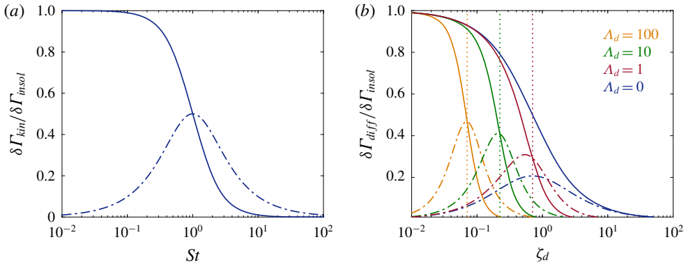
FIGURE 8. (a) Real (solid line) and imaginary (broken line) components of the perturbed surface concentration for kinetically limited adsorption ( Da \rightarrow 0 ) to an oscillating bubble, from (3.44). (b) Surface concentration in diffusion-limited mass transfer ( Da \rightarrow \infty ), from (3.50). \Lambda_d = 0 represents a planar interface following (3.48). The vertical dashed lines show locations where 2\Lambda_d\zeta_d^2 = 1 when \Lambda_d \gtrsim 1 , indicating modified diffusion times for small bubbles via (3.53).
