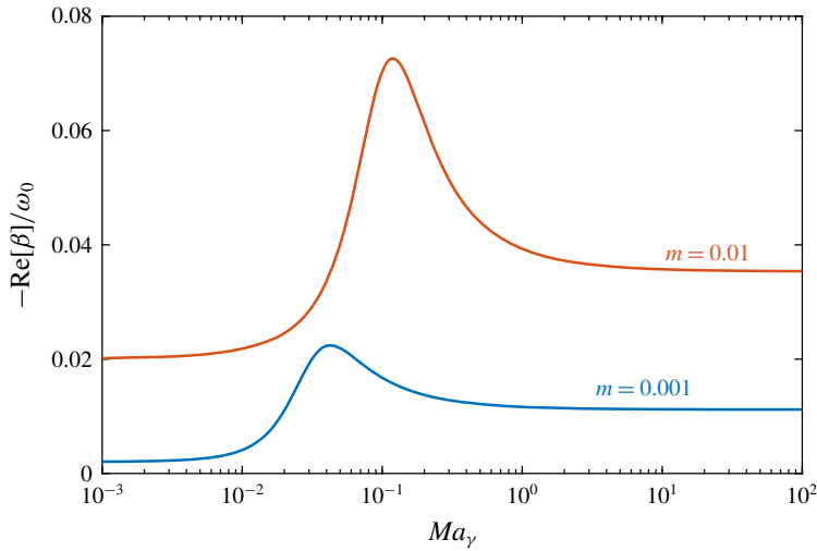
FIGURE 18. Capillary wave damping rate \beta (4.71) as a function of the Marangoni number Ma_\gamma = E_0/\gamma and the normalized fluid viscosity m = \nu k^2/\omega_0 . The damping rate asymptotes to \beta_{clean} = -2m\omega_0 when Marangoni flows are weak ( Ma_\gamma \ll 1 ) and to \beta_{stiff} = -(\omega_0/2)\sqrt{m/2} when the interface is immobilized ( Ma_\gamma \gg 1 ). Waves decay faster in a more viscous fluid (larger m ) for all Ma_\gamma .
