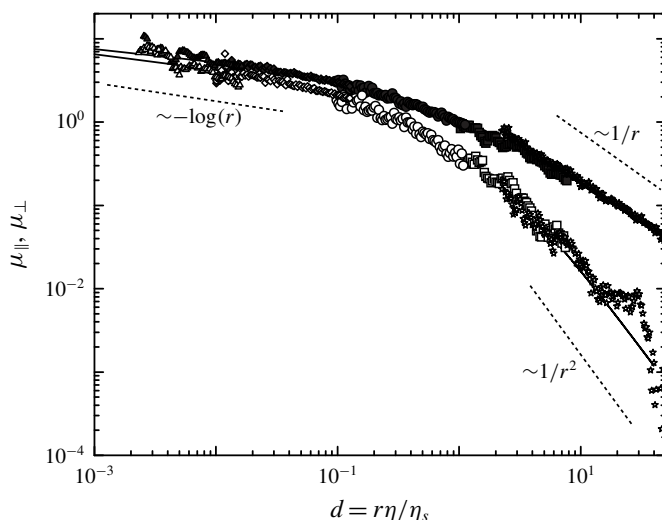
FIGURE 13. Mobility coefficients in the radial ( \mu_{\parallel} ) and azimuthal ( \mu_{\perp} ) directions (in arbitrary units) extracted from two-particle microrheology. In the surface-dominated regime ( Bq \gg 1 or d \ll 1 ), both coefficients decay logarithmically with distance, following (3.112). In subphase-dominated cases ( Bq \ll 1 or d \gg 1 ), the coefficients decay as 1/r and 1/r^2 . The symbols correspond to two-particle displacement correlations along the line of centres (filled symbols) and perpendicular to it (empty symbols), and the solid lines are fits to (3.109). The shapes of the symbols correspond to different surface viscosities. Adapted from Prasad et al. (2006).
