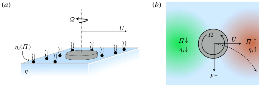
FIGURE 30. Surface ‘Magnus’ effect. (a) A circular particle forced to rotate while translating in a \Pi -thickening surfactant follows a Magnus-like trajectory (b) Surfactant in front of the translating disk has higher surface viscosity than the surfactant behind the disk, owing to the higher surface pressure. Consequently, the rotation of the particle causes it to ‘roll’ upwards, perpendicular to the direction of forcing (Manikantan & Squires 2017a).
