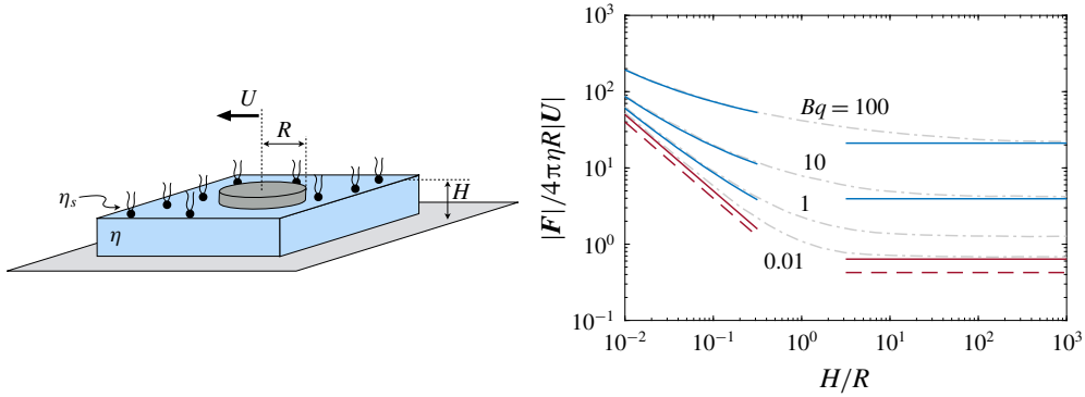
FIGURE 23. A cylindrical disk translating within an insoluble surfactant monolayer atop a bulk fluid layer of finite depth H . Also shown is the resistance coefficient |F|/4\pi\eta R|U| as a function of both sublayer thickness and Boussinesq number. The grey dash-dot lines are the numerical calculations of Stone & Ajdari (1998) at specified Bq , and the solid lines are asymptotic values for small and large H/R . The bottom-most solid lines represent the Bq \rightarrow 0 limit (table 4). The dashed asymptotes correspond to a clean interface, from (4.158) and (4.162), and highlights the fact that even an inviscid surfactant increases drag on a translating probe as compared to a surfactant-free surface.
