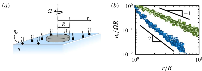
FIGURE 12. (a) A disk of radius R rotating at a constant angular velocity \Omega within a monolayer of surface shear viscosity \eta_s . (b) Surface velocity u_s follows (3.100) when subphase dominant ( Bq \ll 1 , blue squares) and (3.101) when interface dominant ( Bq \gg 1 , green circles); adapted from Zell et al. (2014).
