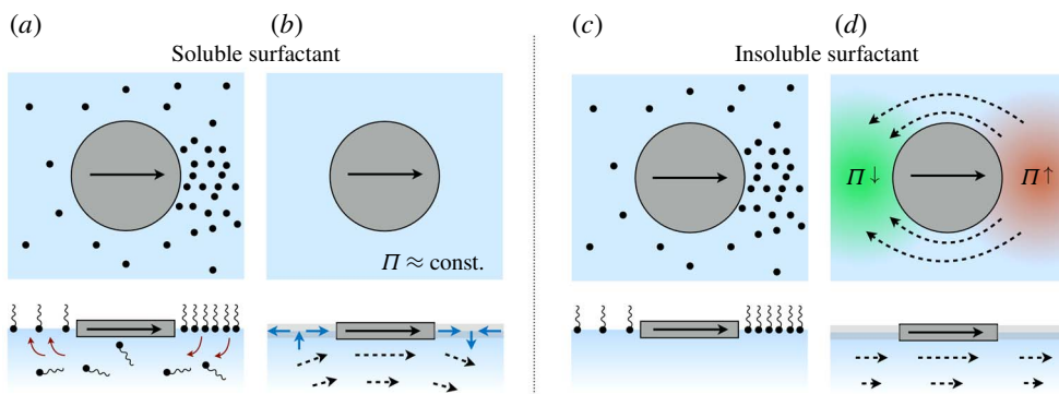
FIGURE 11. Illustration of surfactant-induced incompressibility. (a) Motion of a probe establishes a surface concentration gradient, shown in top and side views. In a soluble monolayer with instantaneous adsorption/desorption, surface concentration gradients are rapidly eliminated. (b) In this limit, \Delta\Pi \approx 0 and reverse Marangoni flows are absent. The surface flow has a non-zero divergence ahead and behind the disk. Bulk fluid flow is indicated by the dashed arrows and is indistinguishable from that corresponding to a stress-free clean interface. (c) By contrast, if the surfactant is insoluble, a surface concentration gradient is sustained, and (d) the surface pressure difference \Delta\Pi generates a reverse Marangoni flow that resists interfacial compression/dilatation. The modified surface flow is divergence free, which changes the bulk flow by constraining it to flow in planes parallel to the interface (see discussion).
