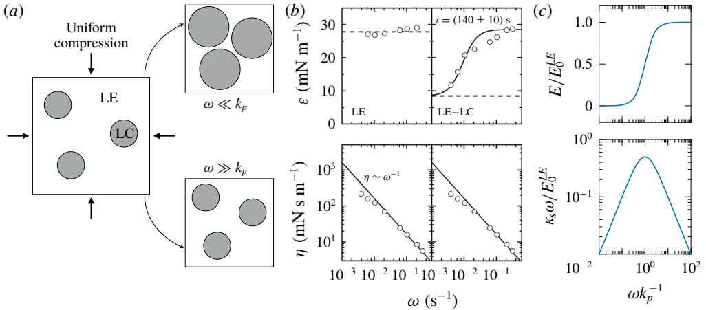
FIGURE 28. (a) Response of a monolayer with coexisting phases to uniform compression: when \omega \ll k_p , domains grow much faster than the rate of compression, and the LE phase offers no elastic resistance. By contrast, when \omega \gg k_p , the rate of compression exceeds the rate of molecules changing phases, and the LE phase offers a net resistance to compression. (b) Measurements of Arriaga et al. (2010) showing elastic and viscous moduli from oscillatory measurements in LE and in coexistence. The solid lines are fit to a Maxwell viscoelastic fluid with characteristic relaxation time \tau = k_p^{-1} \approx 140 s, and the dashed lines are slopes from equilibrium ( \omega \rightarrow 0 ) isotherms. (c) Effective elastic and viscous moduli following (5.16).
