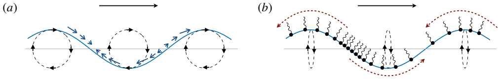
FIGURE 19. (a) Circular motion of interfacial fluid particles on the clean surface of a wave moving to the right. The solid blue arrows along the interface depict compression and expansion of the surface. (b) Surfactants distort circular trajectories via Marangoni flows (red dashed arrows) that oppose the compression and expansion of the interface. The trajectories of fluid elements are then distorted, becoming straight lines in the Ma_\gamma \rightarrow \infty limit.
