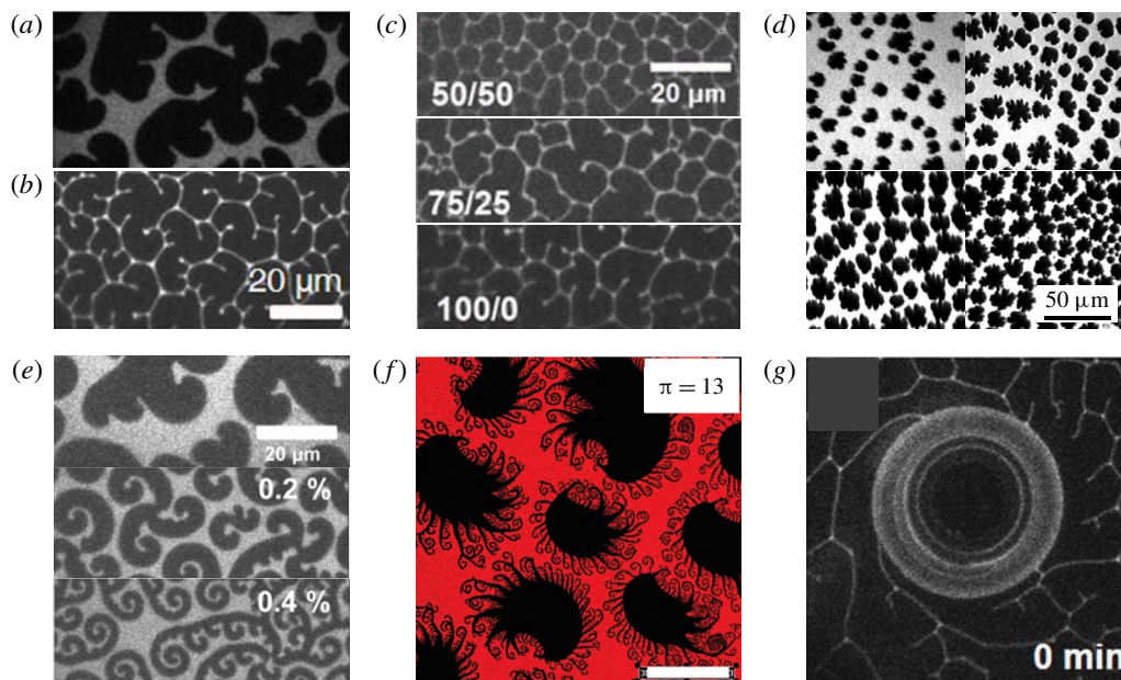
FIGURE 27. (a,b) The phospholipid Dipalmitoylphosphatidylcholine (DPPC) in (a) LC/LE coexistence and (b) polycrystalline, fully LC phase, from Kim et al. (2018). Natural DPPC forms LC domains that wind in a counter-clockwise fashion, owing to the chiral attachment of the two hydrocarbon tails. (c) The chirality of domains within an LC DPPC monolayer depends on the ratio of right- to left-handed DPPC molecules (from Kim et al. (2018)). (d) Palmitic acid co-crystallizes with DPPC to form stiff inclusions, here dispersed by a disordered phase of the unsaturated lipid POPG (from Ding, Warriner & Zasadzinski (2002)). (e) Cholesterol is ‘line active’ for DPPC, promoting the growth of thinner LC grains that wind more tightly (from Kim et al. (2013)). (f) DPPC/hexadecanol/cholesterol mixtures form eerily beautiful grains in LC/LE coexistence, consisting of a DPPC/HD co-crystallized core, surrounded by wispy, spiralling DPPC/cholesterol arms (from Sachan et al. (2017)). (f) An LC-DPPC monolayer that is steadily deformed by a rotating microfabricated ‘button’, reveals a surface yield stress: the monolayer flows within the high-stress region near the button, but is stationary outside a yield radius (from Kim et al. (2018)).
