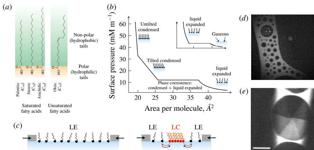
FIGURE 25. (a) Fatty acids consist of a (hydrophilic) carboxylic acid headgroup and a (hydrophobic) hydrocarbon tail. The longer the hydrocarbon tail, the lower its solubility in water and the stronger the van der Waals attractions with adjacent fatty acids. Saturated hydrocarbon tails pack well with each other, whereas unsaturated tails (e.g. oleic acid, with a double bond at the ninth carbon) are ‘kinked’ and frustrate packing. (b) Generalized isotherm of an insoluble monolayer of saturated fatty acids, adapted from Kaganer et al. (1999). Monolayers form a gaseous phase at extremely low concentration (inset), which condenses to form a disordered, liquid expanded (LE) phase when compressed. At higher surface concentrations, a phase transition occurs from the LE phase to one of various liquid condensed (LC) phases with different liquid crystalline order, and even further phase transitions at higher concentrations (here to an untilted, condensed phase). (c) Cartoon showing transition between a disordered, low-density phase (e.g. LE or gaseous) to phase coexistence with a higher-density phase (e.g. LE/LC or gas/LE). (d) Fluorescence micrograph showing gas/LE phase coexistence of the phospholipid DPPC (courtesy of Dr I. Williams). (e) Polarized micrograph of LE–LC phase coexistence between methyl eicosanoate(C 20 ). Within the LC domain, the six different brightness levels correspond to six distinct orientations of the packed tails, which in turn reveal the hexagonal headgroup lattice (from Knobler & Desai (1992)).
