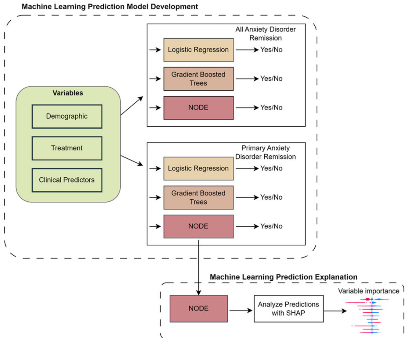
Figure 1. Machine learning prediction model development and explanation.
