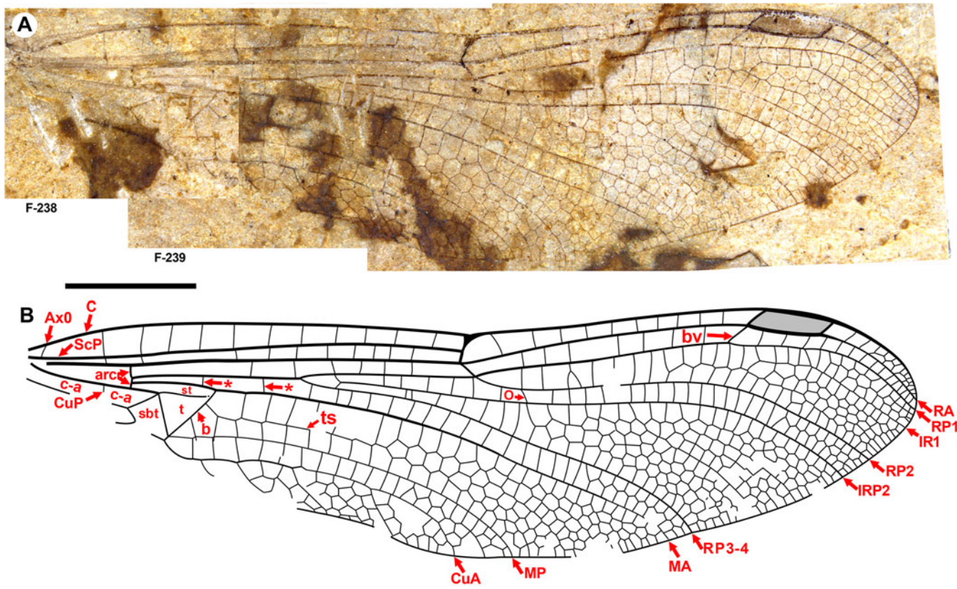
Fig. 12. Auroradraco eos new species, holotype forewing F-238, F-239. A , combination of photograph of F-239, with the basal posterior portion F-238 (regions damaged in F-239); B , drawing from both the part and counterpart. Abbreviations: c-a is the cubito-anal space, see text for other labeling. Both to scale, 5 mm.
