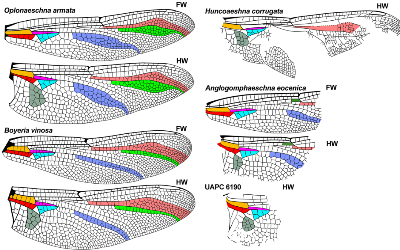
Fig. 4. Further wings of comparative genera of Aeshnidae, see caption for Fig. 2. Extant wings redrawn from Garrison et al. (2006), the Eocene Huncoaeschna corrugata from Petrulevičius et al. (2010), Anglogomphaeschna eocenica from Nel and Fleck (2014), and UAPC 6190 from Wighton and Wilson (1986). FW, forewing; HW, hind wing.
