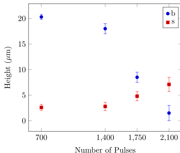
Figure 8. Correlation of remaining substrate thickness b and structure height s for different numbers of pulses. The laser fluence of 5.7 kJ/m 2 and the rotation angle of \Delta\alpha = 45^\circ were kept constant, as well as the ambient medium, which was isopropanol in all cases.
