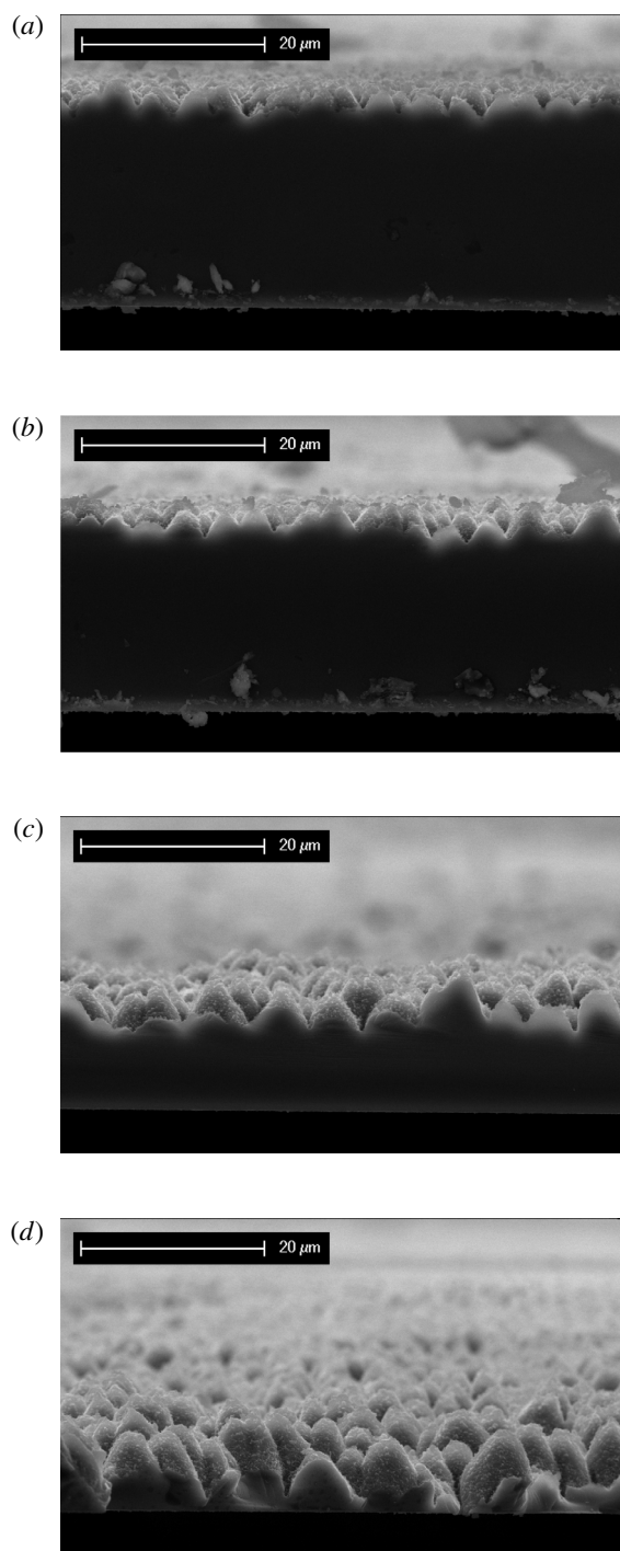
Figure 7. Si wafers processed in liquid isopropanol from an approximate 90° degree side view. The number of pulses were (a) 700, (b) 1400, (c) 1750 and (d) 2100 respectively, with a constant rotation angle of \Delta\alpha = 45^\circ . The laser fluence of 5.7 kJ/m 2 was kept the same.
