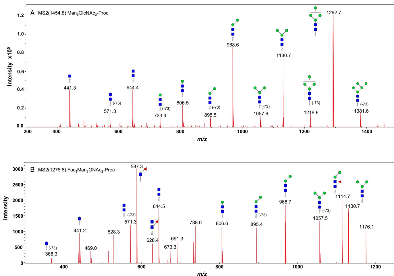
Fig. 7. Positive-ion MS/MS spectra of Man 5 GlcNAc 2 -Pro (A) and Fuc 1 Man 3 GlcNAc 2 -Pro (B) from O. ochengi GST1. (-73) refers to [M + H] + ions that have lost terminal diethylamine from the procainamide tag during the collision (Kozak et al. , 2015). Blue squares, N-acetylglucosamine residues; green circles, mannose residues; red triangles, fucose residues; Proc, procainamide tag.
