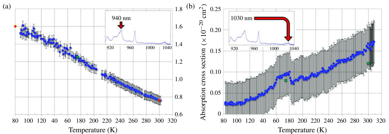
Figure 2. The thermal evolution of the absorption cross section between 90 and 300 K for an HDC grown homogeneously 1 at.% doped 1 cm thick Yb:YAG crystal. The data in (a) are collected at 940 nm whereas those in (b) correspond to the 1030 nm absorption peak. The red dots refer to data from Fan [7] whereas the green ones refer to data from Brown [8] .
