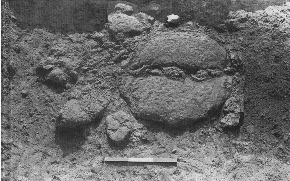
A. Stone-setting (crushing-platform) F 317 from the east at Woolaston. Scale: 0.3 m. (p. 177) (Photo: M.G. Fulford)
