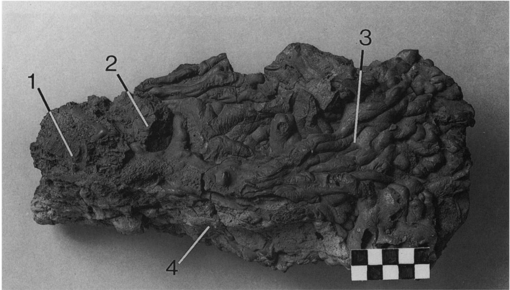
A. Iron-making residue at Woollaston: slag mass from dump: 1. massive slag. 2. piece of incompletely reacted ore. 3. sheets of tap slag (flow to right). 4. wall of baked clay. Scale in centimetres. (p. 193)
