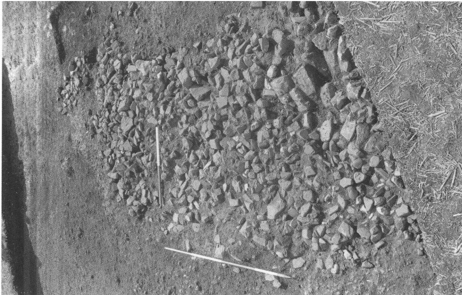
(Photo: J. L. Watkins) B. Iron-making residue at Woolston: slag mass from dump: 1. pool of slag; 2. massive slag with ore and charcoal; 3. rib of baked clay, glassy and vesicular to right (furnace interior); 4. sheets of tap slag (flow to left). Scale marked in centimetres. (p. 193)
