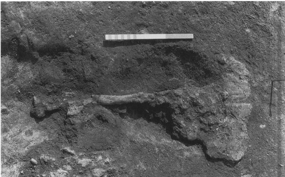
B. Remains of Iron-making Furnace F 19/20 at The Chesters villa, Woolaston, Glos.: remains of furnace to right and slag pool with chilled 'finger' of slag centre and left. Scale: 0.3 m. (pp. 169, 193)
