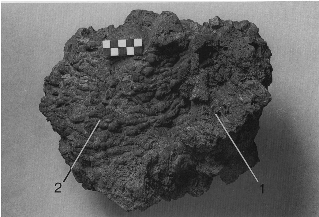
B. Iron-making residue at Woollaston: slag mass from dump: 1. massive slag with incompletely reacted ore and charcoal. 2. sheets of tap slag (flow to left). Scale in centimetres. (p. 193)
