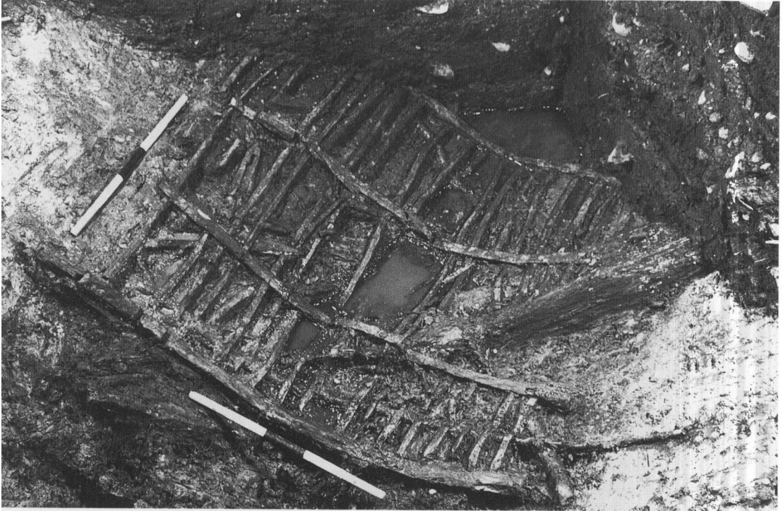
A. Carlisle: Possible cage side (Wood No. 27) as found. Scales 50 cm long. (p. 76)
