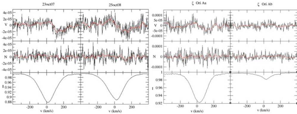
Figure 1. Left: Examples of I (bottom), null N (center) and Stokes V (top) profiles for two nights. Right: I (bottom), null N (center) and Stokes V (top) profiles for October 25, 2008, for ζ Ori Aa (left) and ζ Ori Ab (right). The red lines represent the averaged signal.
