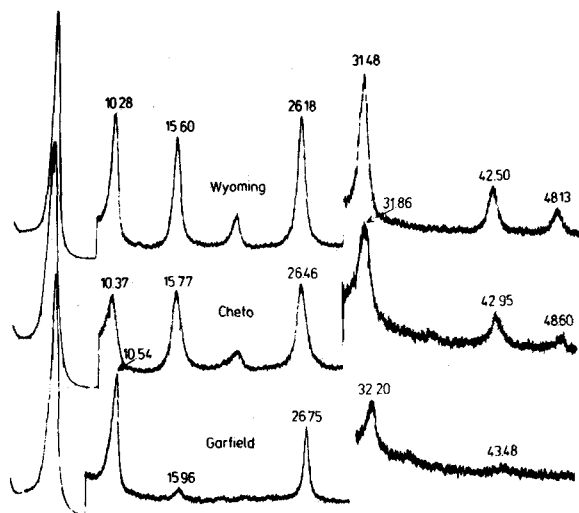
Figure 1. Examples of X-ray powder diffraction patterns of glycolated smectites. 2\theta values for \text{CuK}\alpha radiation are listed by important peaks. 2\theta values of 00\ell reflections of the Cheto and Garfield samples are regularly shifted with respect to Wyoming, suggesting smaller ethylene glycol-smectite complex thickness.
