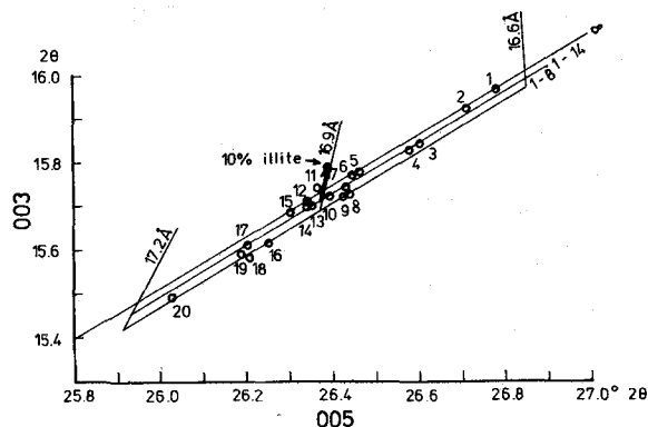
Figure 2. Plot of 2\theta(003) vs. 2\theta(005) for variable ethylene glycol-smectite thickness. The three lines represent an infinite number, 1–14, and 1–8 layers/domain. The calculated position of a 10/90 is plotted to show the effect of mixed layering. 1 = Garfield, Washington, Ward's Natural Science Establishment; 2 = Uruguay, Ralph Grim collection; 3 = Polkville, Mississippi, Ward's Natural Science Establishment; 4 = No. 30, Ralph Grim collection; 5 = Chmielnik, Poland; 6 = EU-3-75, Wisconsin, Ralph Grim collection; 7 = Black Jack Mine, Idaho, Smithsonian Collection; 8 = Otay, California, Ward's Natural Science Establishment; 9 = hectorite, Hector, California, SHCa-1, CMS Source Clays Repository; 10 = Piasczno, Poland; 11 = Cheto, Arizona, SAz-1, CMS Source Clays Repository; 12 = Milos, Greece, Ralph Grim collection; 13 = saponite, Riddle, Oregon; 14 = Montmorillon, France, Ralph Grim collection; 15 = Wiślica, Poland; 16 = No. 222, Ralph Grim collection; 17 = Machów, Poland; 18 = Gacki, Poland; 19 = Crook County, Wyoming, SWv-1, CMS Source Clays Repository; 20 = Umiat, Alaska.
