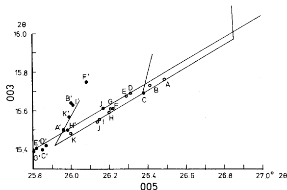
Figure 3. Projection of synthetic, glycolated, dioctahedral montmorillonites and beidellites onto 003 vs. 005 plot. Open circles = Mg-minerals; solid circles = K-minerals.
