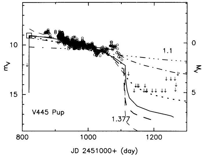
Fig. 3. Same as figure 2 but its enlargement. 1.1 (dash-three-dotted), 1.2 (dash-dotted), 1.3 (dotted), 1.33 (solid), 1.35 (dashed), and 1.377 M_{\odot} (thin dashed). The theoretical curves except 1.33 M_{\odot} are shifted in the vertical direction: 1.5, 1.5 and 0.5 mag upward for 1.1, 1.2 and 1.3 M_{\odot} and 0.2 and 0.9 mag downward for 1.35 and 1.377 M_{\odot} , respectively.
