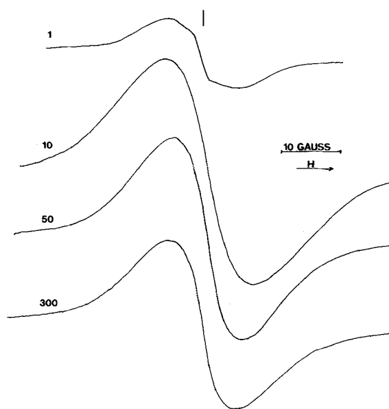
Figure 5. Electron spin resonance spectra of dry tetramethyl benzidine-treated hectorite films (1, 10, 50, and 300 mmole/100 g).
