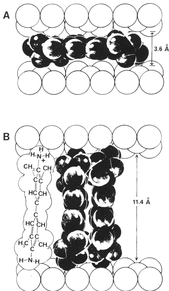
Figure 6. Proposed interlamellar alignment of tetramethyl benzidine for (A) 13.2-Å hectorite complex and (B) 21-Å hectorite complex.
