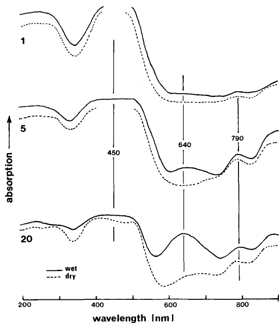
Figure 2. Ultraviolet-visible reflectance spectra of wet and dry hectorite films treated with 1, 5, and 20 mmole tetramethyl benzidine/100 g.
