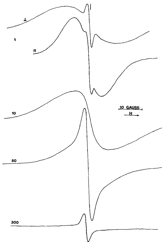
Figure 4. Electron spin resonance spectra of moist tetramethyl benzidine-treated hectorite films (1, 10, 50, and 300 mmole/100 g). Free electron ( g = 2.0023 ) position is indicated by vertical marker.
