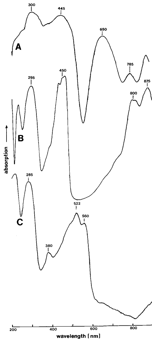
Figure 3. Ultraviolet-visible spectrum of tetramethyl benzidine: A. Adsorbed on dry hectorite film at 300 mmole/100 g level (reflectance spectrum); B. Dissolved in methanol and oxidized by manganese oxide (absorbance spectrum); C. Adsorbed on hectorite in aqueous suspension to form "red" complex (10 mmole/100 g) (absorbance spectrum).
