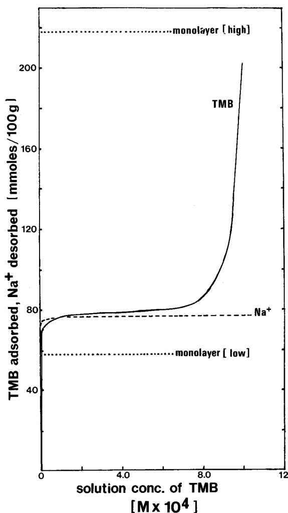
Figure 1. Adsorption of tetramethyl benzidine (TMB) and desorption of Na + as function of equilibrium concentration of TMB in aqueous solution. Calculated quantity of TMB required for monolayer coverage of hectorite interlayers based upon molecular dimensions of TMB are indicated for horizontal (low) and vertical (high) molecular orientations.
