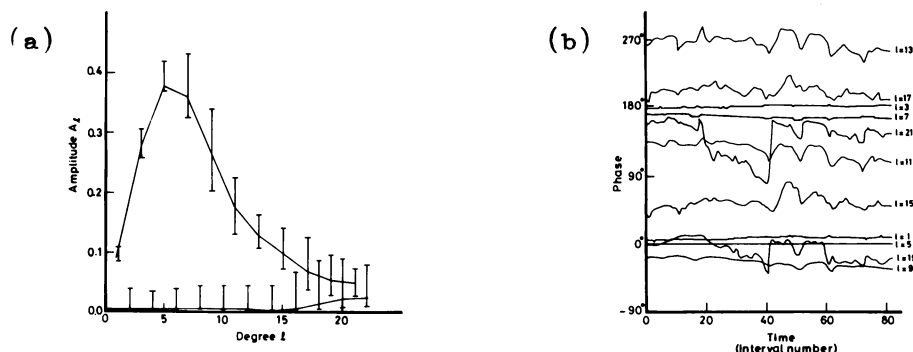
Figure 1. (a) Spectrum of relative amplitudes of the axisymmetric modes of 22y periodicity in 'B \phi '. The bars represent total scatter of the 82 values corresponding to the 82 intervals. The continuous curve represents the values obtained from the whole data set of the 103 years. (b) Relative phases (\varphi_l - \varphi_5) .
