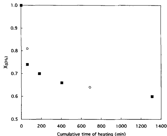
Figure 2. The fraction of hydrogen, X_S(H_2) , remaining in the sample plotted against the cumulative time of heating (at 250°C) for halloysite 1, experiment MHD-1945 (■) and for halloysite 2, experiment MHD-1950 (○). The rate of H loss (evolved as water) decreases with time. Despite different total water contents (see footnote to Table 1), between 36–40% of the structural hydrogen of the OH group (reported as water) is lost from both samples after \sim 685 min of heating at 250°C in vacuo .
