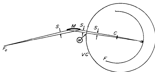
Fig. 1. Schematic experimental arrangement, F_0 : X-ray focus, M : doubly bent monochromator, S : slit, C : Crystal, F : film, VC : vacuum chamber, W : Be-window.
