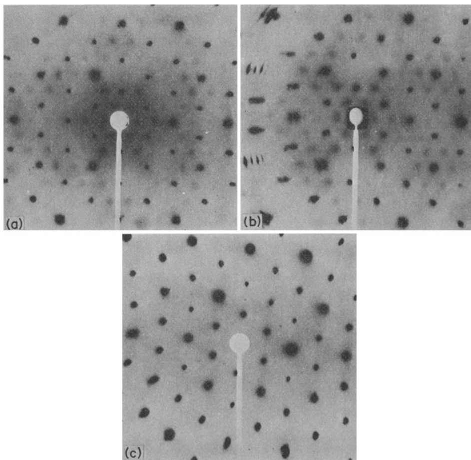
Fig. 3. Ni-vermiculite, X-ray diffraction photographs. (a) Hydrated specimen with the crystal perpendicular to the X-ray beam (b) Hydrated specimen with the crystal at 20^\circ to the X-ray beam (c) Dehydrated specimen.
