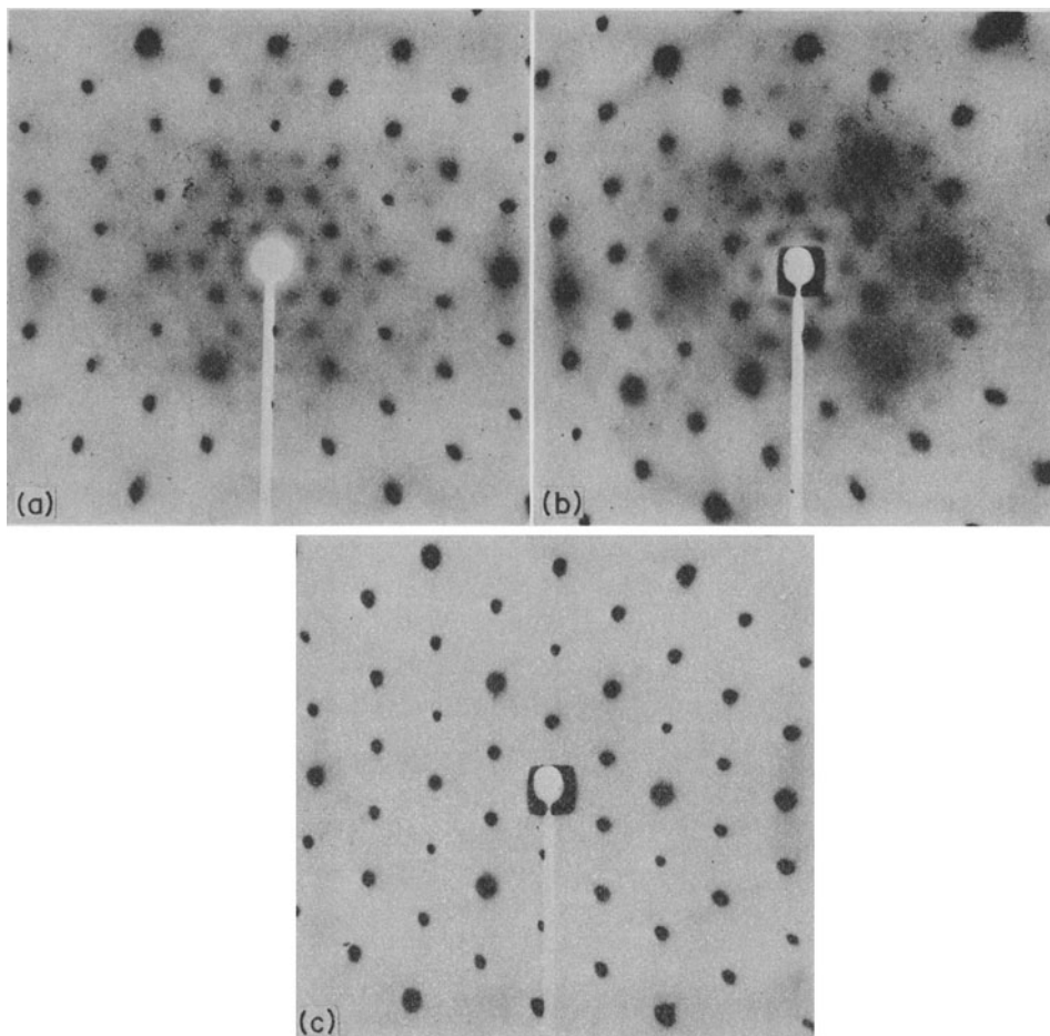
Fig. 2. Mg-Vermiculite, X-ray diffraction photographs. (a) Hydrated specimen with the crystal perpendicular to the X-ray beam. (b) Hydrated specimen with the crystal at 20^\circ to the X-ray beam (c) Dehydrated specimen.
