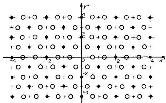
Fig. 4. Projection of the reciprocal space on the X^*Y^* plan. Black circles are the projections of Bragg spots, white circles are the projections of linear diffusions.
