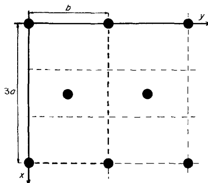
Fig. 5. Patterson section in the interlamellar space obtained from Fourier transform of the preceding projection. The cations are distributed at the apex of 3a, b or (3a + b)/2 vectors (black circles).
