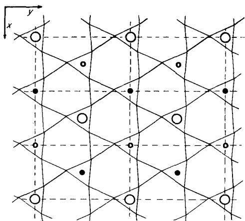
Fig. 6. Mg or Ni cation distribution in a domain. The cations are distributed on a centered lattice of 3a , b parameters (large circles). In the neighboring domains, the cations may occupy one of the two other positions (black and white small circles).
