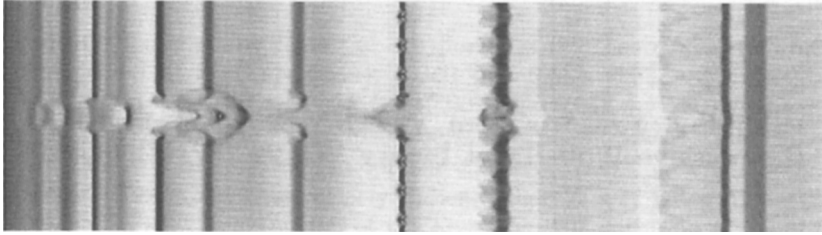
Figure 1. The flow density in the expansion of a small perturbation a line driven wind in a box 1 R_* tall that extends from 1-4 R_* . Variations can be seen in the shadow of the initial perturbation, while away from the shadow, thin shell instabilities can be seen forming. This was calculated on a fixed grid of 800 \times 400 cells, using a modified version of the hydrodynamical code VH-1 (Blondin 1990). The maximum density is \sim 2 \times 10^{-11} \text{ g cm}^{-3} .
