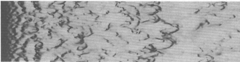
Figure 2. The same piece of photosphere at a later time. Note that while the flow can still be characterised as the ejection of successive shells of dense material, the shells are highly fragmented and limited in extent.
