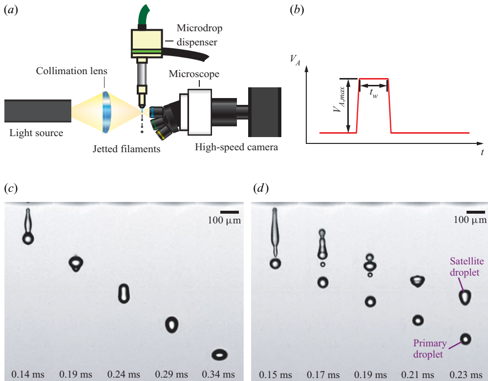
Figure 1. (a) Schematic of the experimental set-up. (b) Typical trapezoidal pulse used for actuation. (c) Jetting with water at V_{A,max} = 50 V, t_w = 40 \mu s results in a single droplet. (d) Jetting with water at V_{A,max} = 60 V, t_w = 40 \mu s results in the formation of a primary droplet and a satellite droplet.
