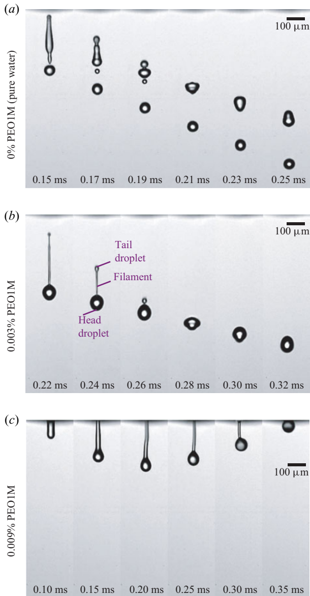
Figure 2. (a) Jetting with water at V_{A,max} = 60 V, t_w = 40 \mu s results in the formation of a satellite droplet ('satellite' regime). (b) Jetting with 0.003 % PEO1M solution ( \lambda = 28.2 ms, c/c^* = 0.022 , nozzle Deborah number ( De_n ) = 1.91) at V_{A,max} = 60 V, t_w = 40 \mu s results in the suppression of satellite droplet formation ('no satellite' regime). (c) A 0.009 % PEO1M solution ( \lambda = 99.38 ms, c/c^* = 0.067 , De_n = 6.75 ) at V_{A,max} = 60 V, t_w = 40 \mu s results in no detachment of droplets from the nozzle ('no jetting' regime).
