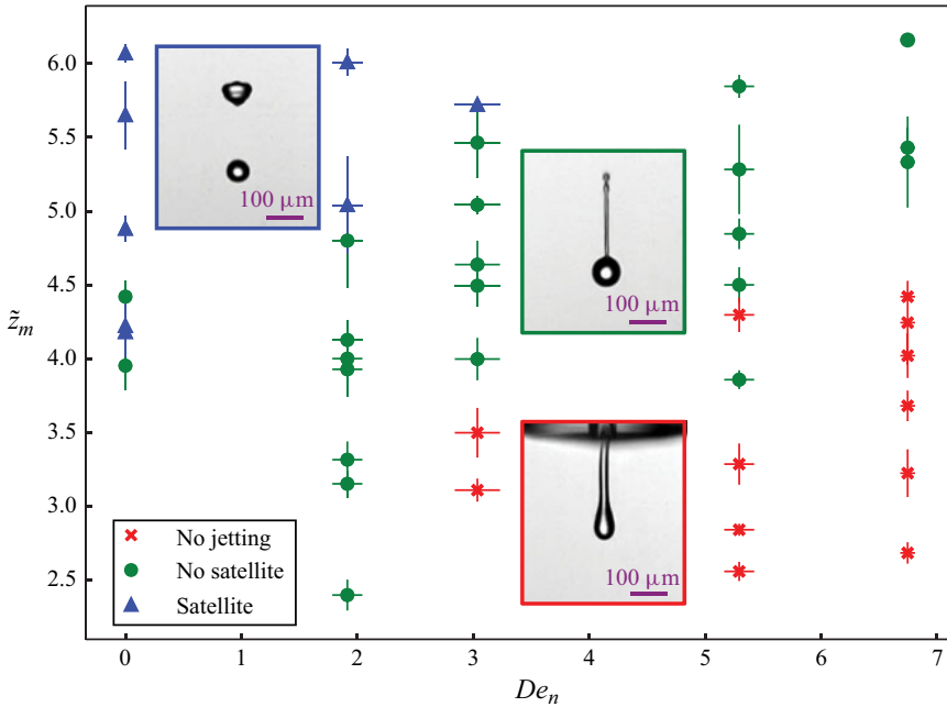
Figure 4. Regime map based on the nozzle Deborah number ( De_n ) and the non-dimensional maximum meniscus position ( \bar{z}_m ). The insets show the typical jetting (or lack of) behaviour observed in each regime, namely satellite formation (blue markers) for low De_n and high \bar{z}_m , no satellite formation (green markers) for intermediate De_n and \bar{z}_m , and no jetting (red markers) for high De_n and low \bar{z}_m . Each datapoint represents approximately 25 experiments.
