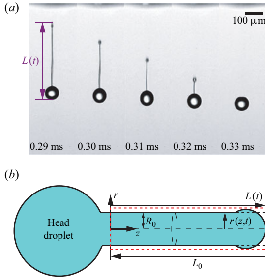
Figure 6. (a) The evolution of a jetted 0.005 % PEO1M ligament produced at V_{A,max} = 60 V, t_w = 40 μs. (b) Schematic of the geometry for the theoretical model, also clarifying the employed notation.
