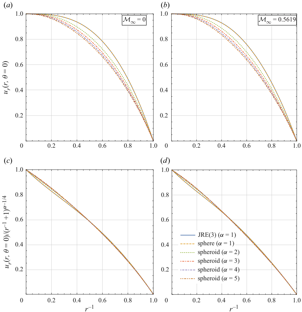
Figure 5. Incompressible (a,c) and critical (for the sphere: \mathcal{M}_\infty = 0.5619 ; b,d) flows in front of the different prolate spheroids of figure 4 (legend), showing the normalized velocity u (a,b) and the scaled velocity u_r/(r^{-1} + 1)^{\alpha-1/4} (c,d). Results are based on the pseudospectral code with a converged (better than line width), (k_{\max}, n_{\max}) = (8, 8) resolution, for \gamma = 7/5 . In the bottom row, we also plot the third-order JRE around a sphere (JRE(3), solid blue), for comparison.
