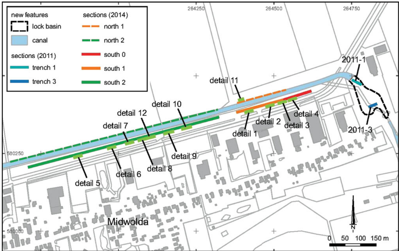
Fig. 3. Map of study area showing the location of the 2011-1 (WP-1), 2011-3 (WP3) and 2014 trenches. The large 2014 trench is subdivided into 'north 1', 'north 2', 'south 0', 'south 1' and 'south 2' parts, of which the latter 'south' parts have been investigated in this study.
