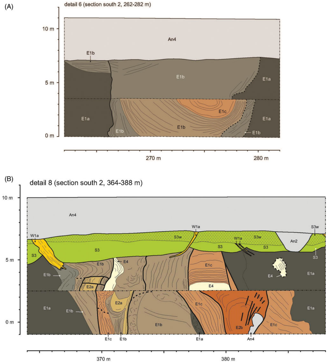
Fig. 7. (A) Lithostratigraphy and glaciotectionics of Elsterian sediments of trench 2014 south 2, detail 6. Synclinal structure with sandy clays (E1b) and sands (E1c) in the core of the structure. (B) Lithostratigraphy and glaciotectionics of Elsterian (units E) and sediments of trench 2014 south 2, detail 8: the layered units have a near-vertical attitude, caused by continuous compressional folding causing overprinted folding and attenuated layering.
