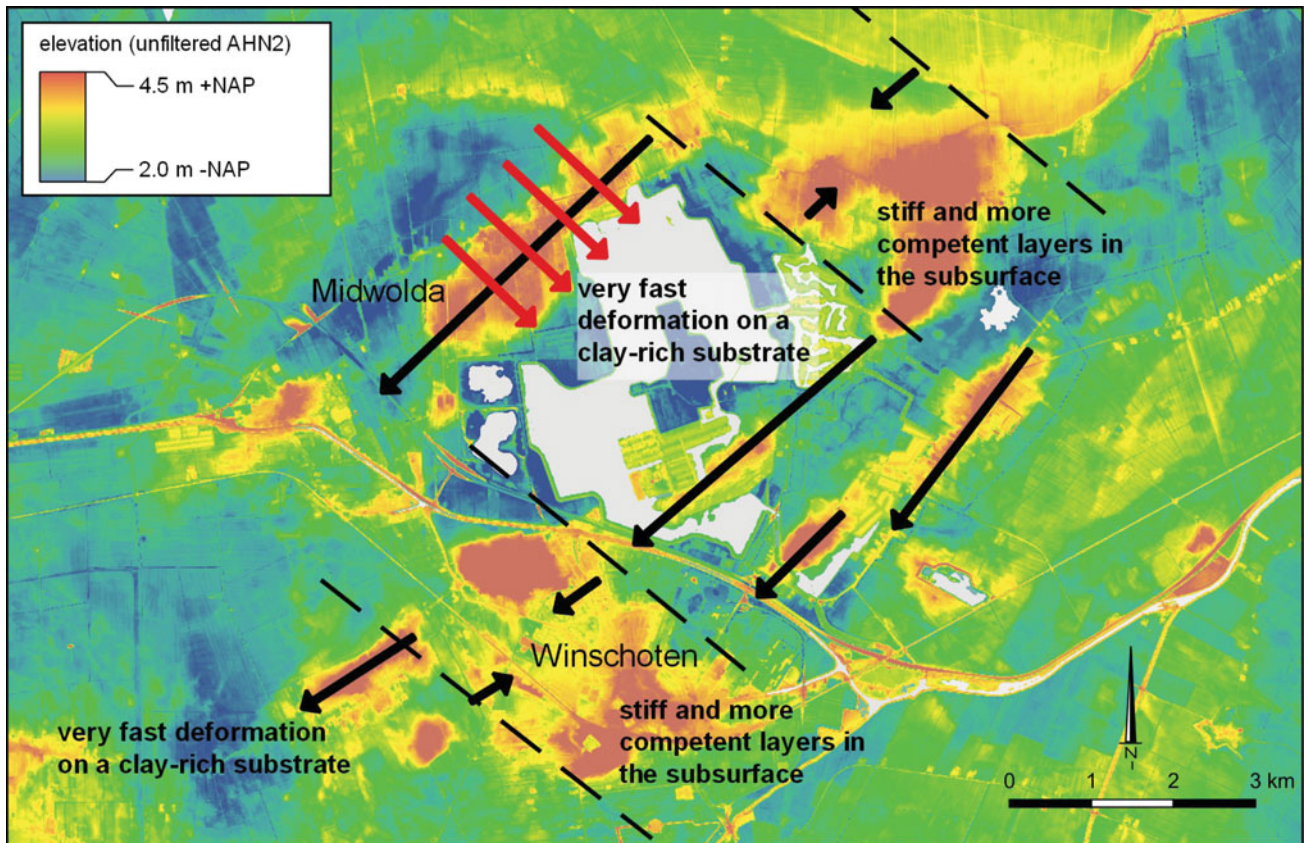
Fig. 15. Substrate-controlled glacial morphology reconstruction based on DEM and the results of this study. Zones with stiff and more competent layers in the subsurface show compressional pushed structures and are alternating with zones with an incompetent clay-rich substrate that show elongated isolated lineations all oriented towards a NE–SW ice-flow regime. The dashed lines represent the separation between the extensional and compressional zones. The short thick black arrows represent the direction of glaciotectionic shortening. The long black arrows represent elongated lineations like the Midwolda ridge. Superimposed, observed in the Midwolda ridge, are NW–SE lineations (red arrows) with associated till deposits that are classified as the Assen Group till (Rappol, 1987; Rappol et al., 1991) with an Eastern Baltic gravel assemblage.
