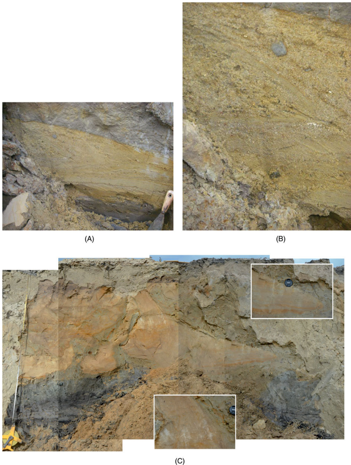
Fig. 11. (A) Medium-scale sheath fold structure within the upper till layer (2011-3 pit). Sheath fold structure has a sand lithology. (B) Detail of the characteristic 'eye' structure of fine-grained 'loamy' layering in the central part of the sheath fold structure (2011-3 pit). (C) Large-scale sheath fold structure in the upper till layer overprinted by a dark-grey type 2 intrusion in the lower left corner see also overview in (A). The centre bottom inset shows near-vertical layering in the 'eye' of the sheath fold; the right upper inset shows first phase of sheath folding of the sand in the upper till. (D) Schematic section showing upper till with large sheath fold (S5) consisting of sand lithology, overprinted by a younger intrusion (S6, 6a) that appears to originate from the basis of the sheath fold structure (2014 pit).
