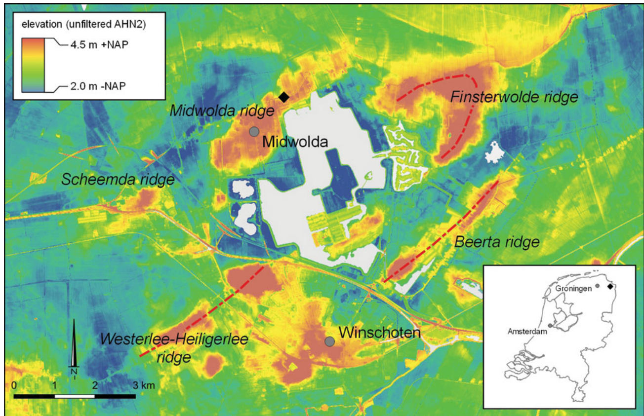
Fig. 1. Digital elevation map of the glacial landscape of eastern Groningen. The Midwolda ridge is located in the north, all other glacial ridges as red dashed lines. The map shows a dominant NE-SW orientation of the elongated relief next to irregular non-oriented relief forms in the NE and SW part of the map ( www.ahn.nl/viewer ).
