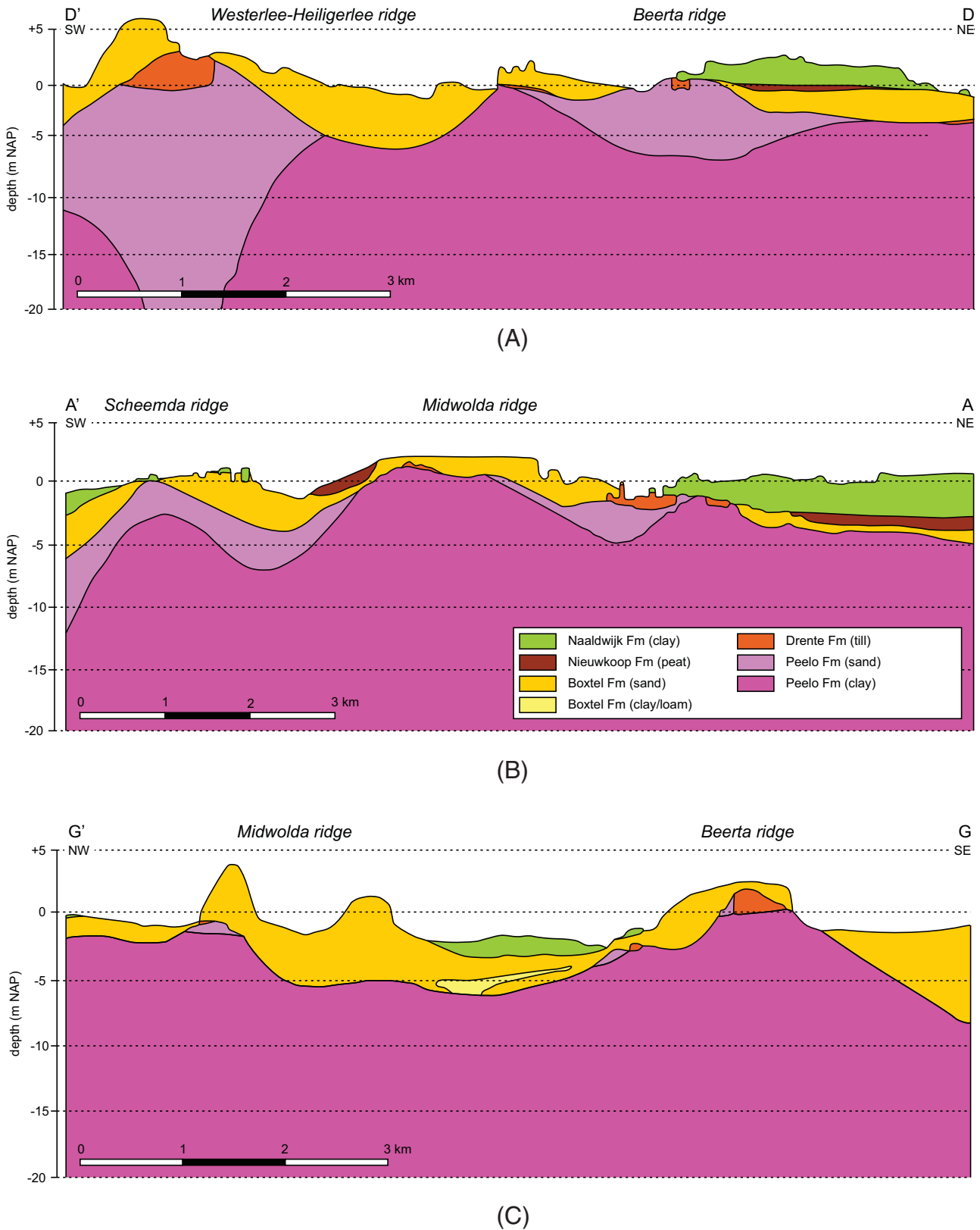
Fig. 13. (A) D-D' NE-SW cross-section shows ridge of Beerta with isolated plug of sandy Peelo Formation and Drente Formation (till) and the Westerlee-Heiligerlee ridge with thick isolated plug of sandy Peelo Formation. (B) A-A' NE-SW cross-section shows Midwolda ridge with small isolated plug of sandy Peelo Formation covered with Drente Formation (till) sloping upwards to the SW. (C) G-G' SE-NW cross-section shows Beerta and Midwolda ridges showing relatively steep slope on the SE part of the Peelo clay, as well as the shallow (5 m deep) basin between both ridges.
