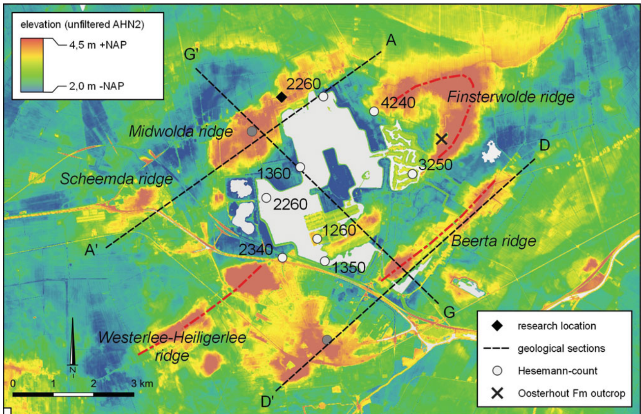
Fig. 12. Overview of Regis II v2.2 cross-sections Finsterwolde–Winschoten (Fig 13A–C) and Hesemann countings of erratic boulders in the vicinity of the Midwolda ridge; X indicates location of exposure of the Oosterhout Formation.
