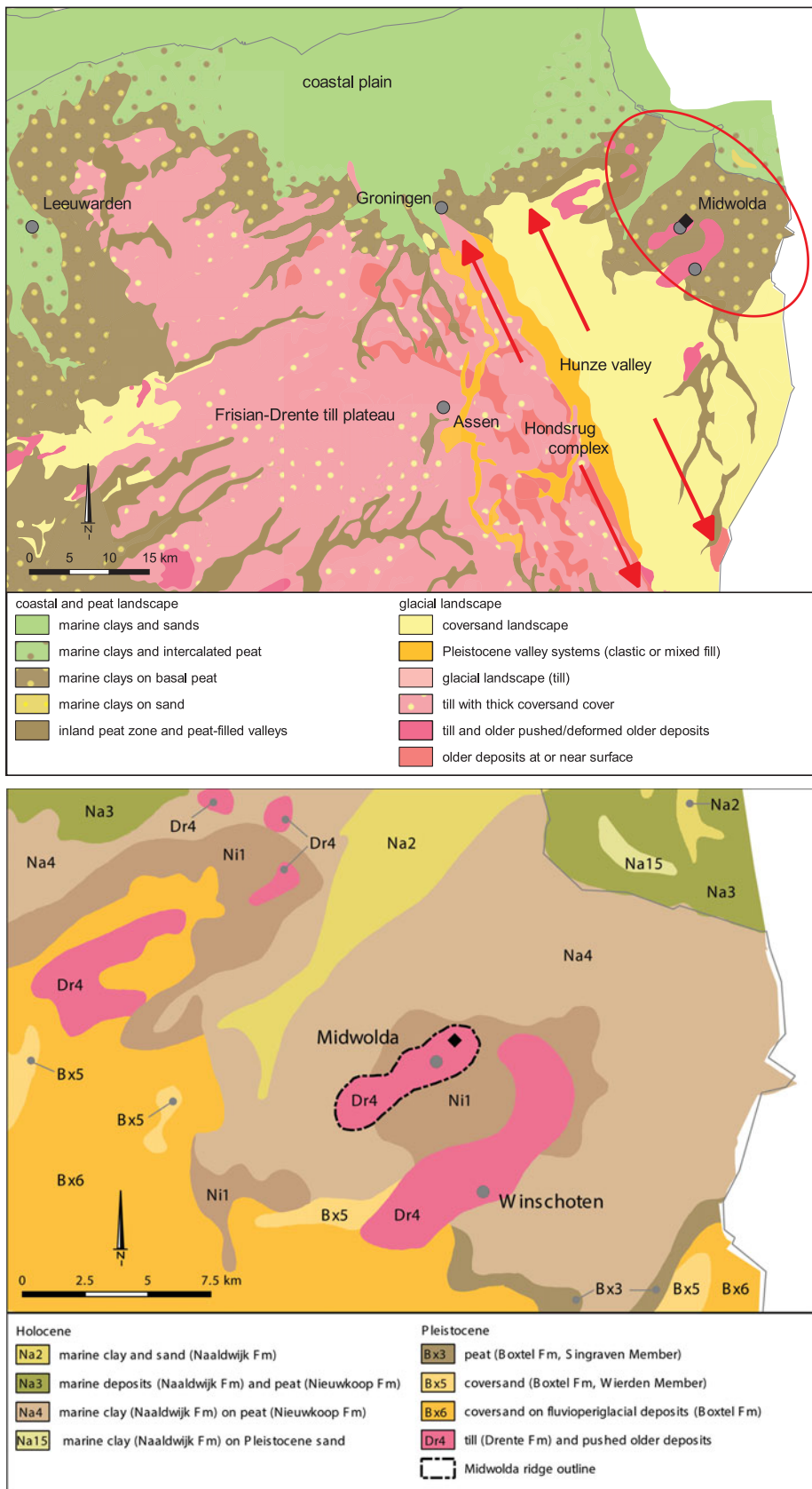
Fig. 2. (A) Simplified geological map of the NE Netherlands showing the main landscape units associated with the Saale glaciation. Red arrows indicate NNW–SSE orientation of Hondsrug ridges and Hunze valley (modified after De Mulder et al., 2003). (B) Geological map of the study area. The Midwolda ridge is marked with a black contour. (Source: DINOLOket/De Mulder et al., 2003.)
