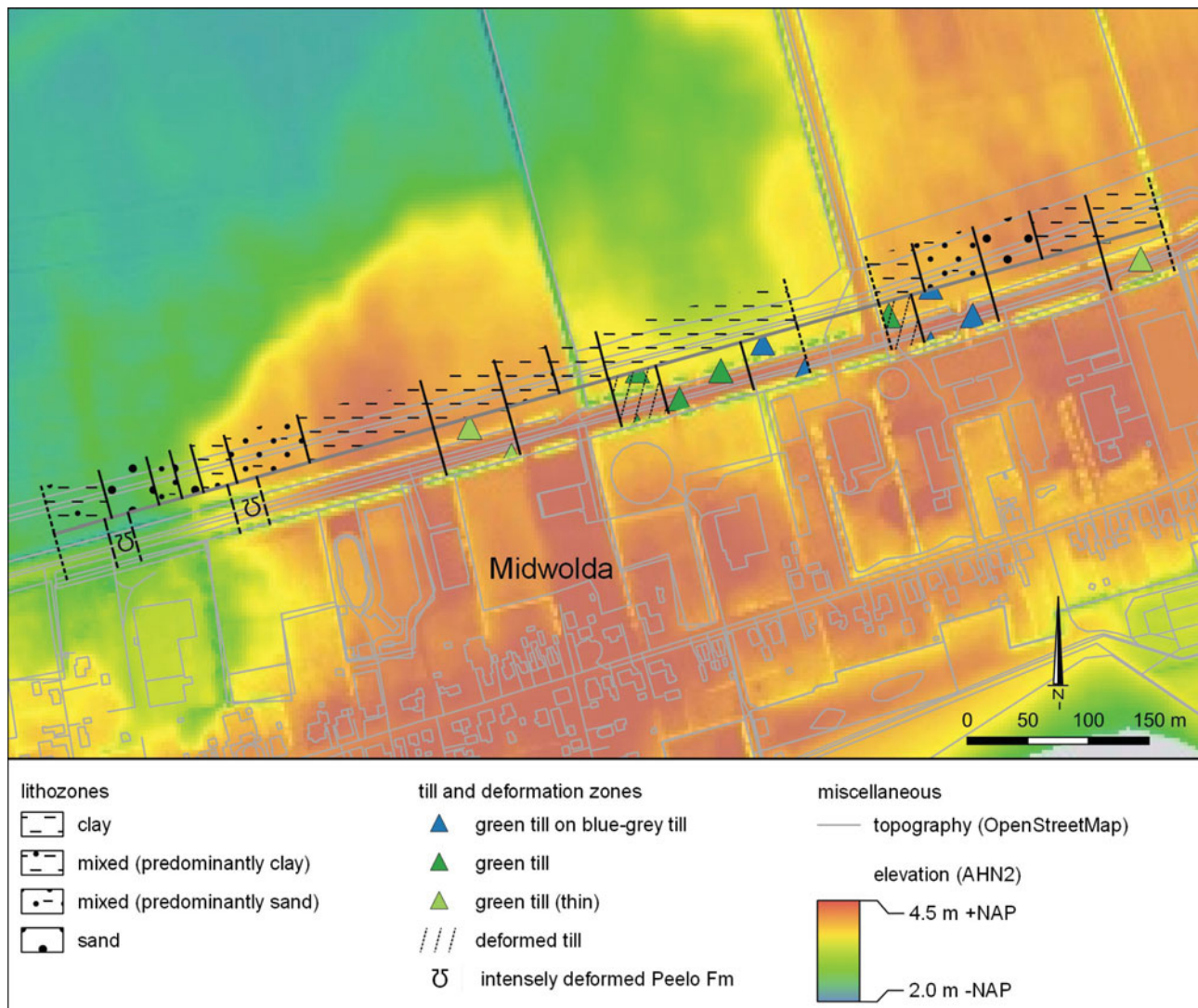
Fig. 14. Structural and lithological map of Midwolda ridge showing lateral distribution of glacial tills as well as structural and lithological characteristics of Elsterian sand and clay.
