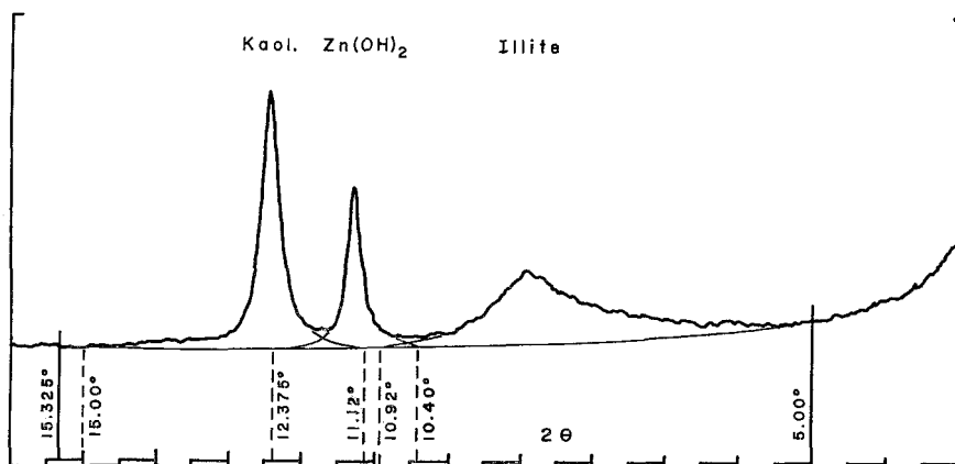
FIG. 3. Diffractometer chart for a standard mixture of equal amounts of kaolinite and illite, showing allocation of base line and peak areas.
