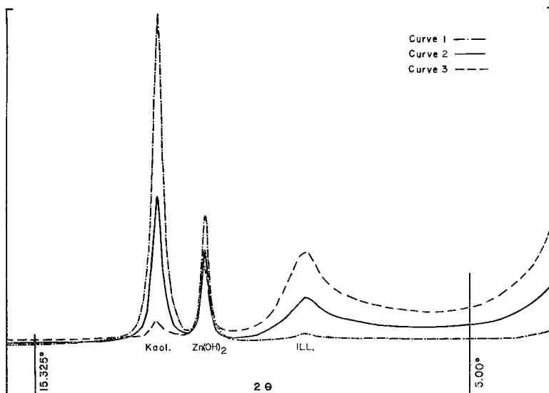
FIG. 2. Superimposed diffractometer charts for three standard mixtures having a constant weight percentage of \text{Zn}(\text{OH})_2 .
