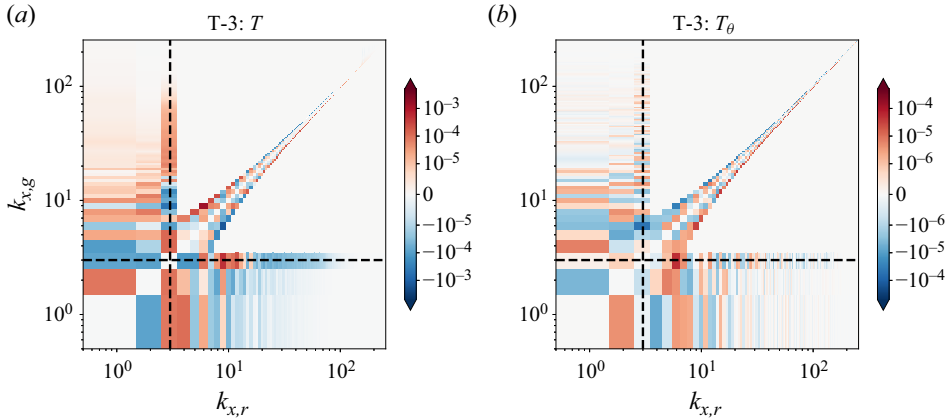
Figure 17. Transfer functions: (a) T(k_{x,r}, k_{x,g}) showing the scale-to-scale kinetic energy transfer and (b) T_{\theta}(k_{x,r}, k_{x,g}) showing the scale-to-scale thermal energy transfer from the T-3 simulation. The horizontal and vertical dashed lines correspond to the threshold wavenumber, k_0 .
