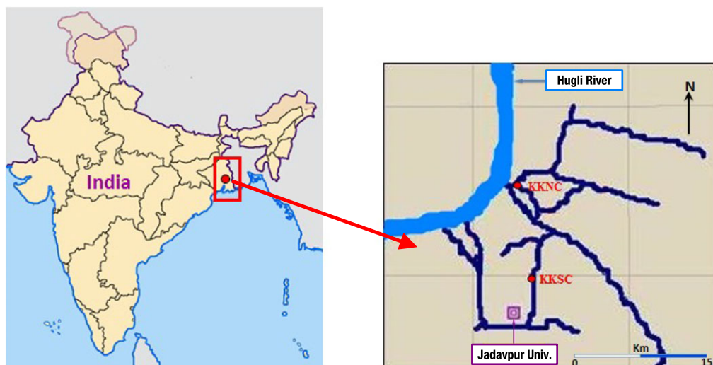
Figure 1 Map of the sampling locations of surface sediments in north and south canals (KKNC and KKSC) and air samples (Jadavpur University) around the city of Kolkata, India.
