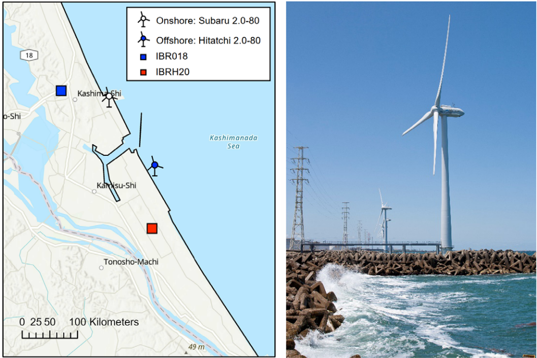
Figure 10. Photograph of the Kamisu (Hasaki) wind farm following the 2011 Tohoku earthquake.
